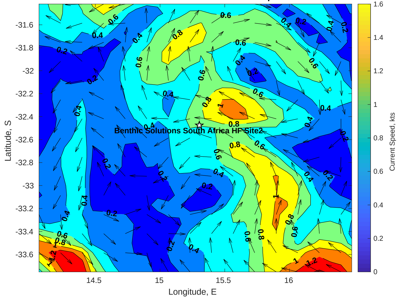
Surface Currents for Benthic Solutions South Africa HF Site2 at 06-Apr-2025 00:00:00
