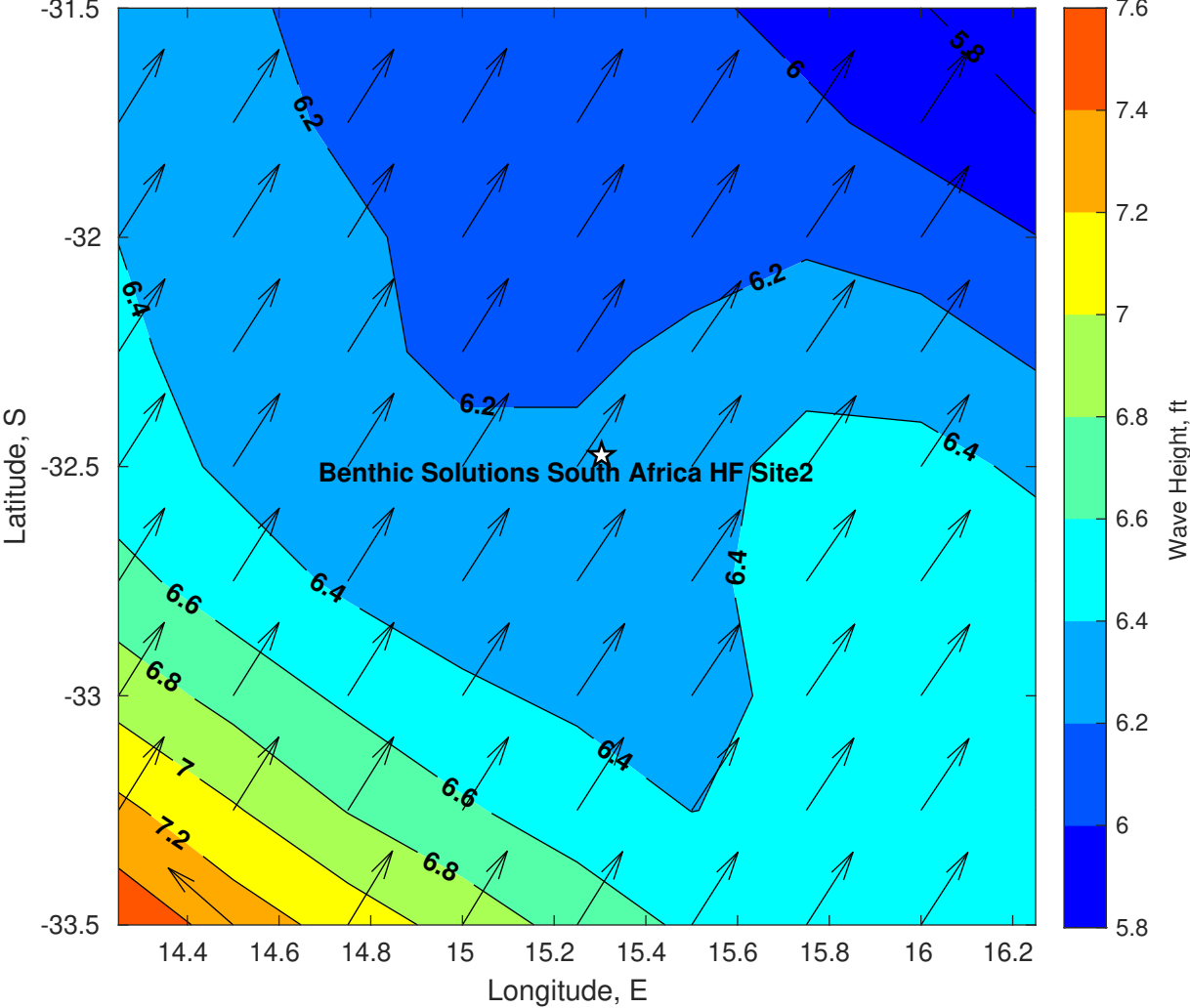
Wave Height (ft) for Benthic Solutions South Africa HF Site2 at 07-Apr-2025 09:00:00
