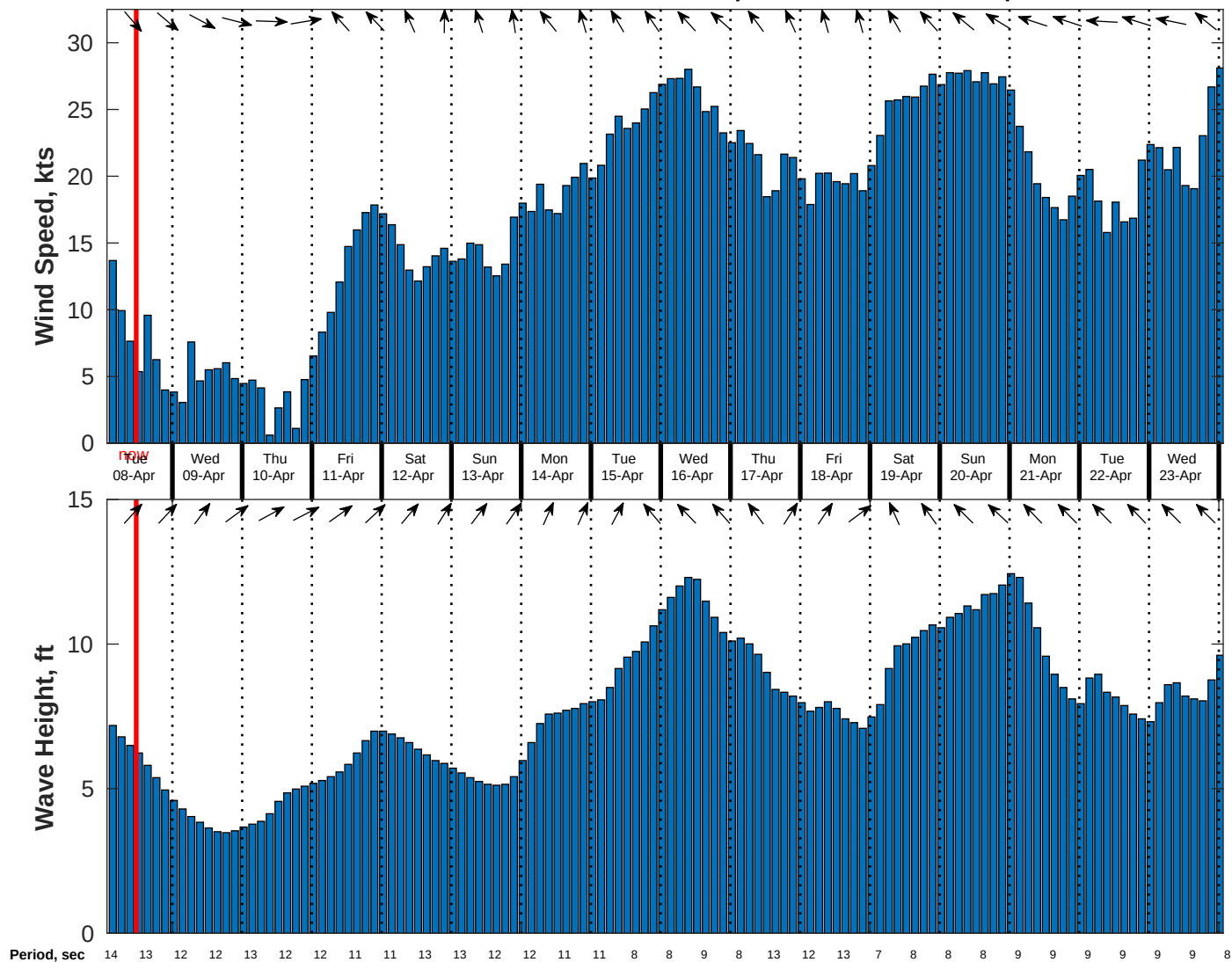
Wind & Wave Forecast for Benthic Solutions South Africa HF Site2 from 07-Apr-2025 02:00:00 to 23-Apr-2025 02:00:00
