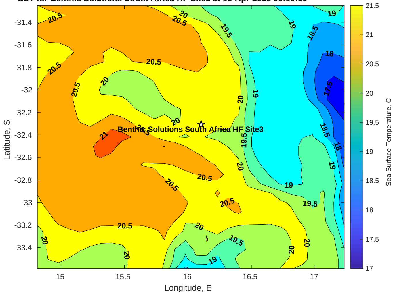
SST for Benthic Solutions South Africa HF Site3 at 06-Apr-2025 00:00:00
