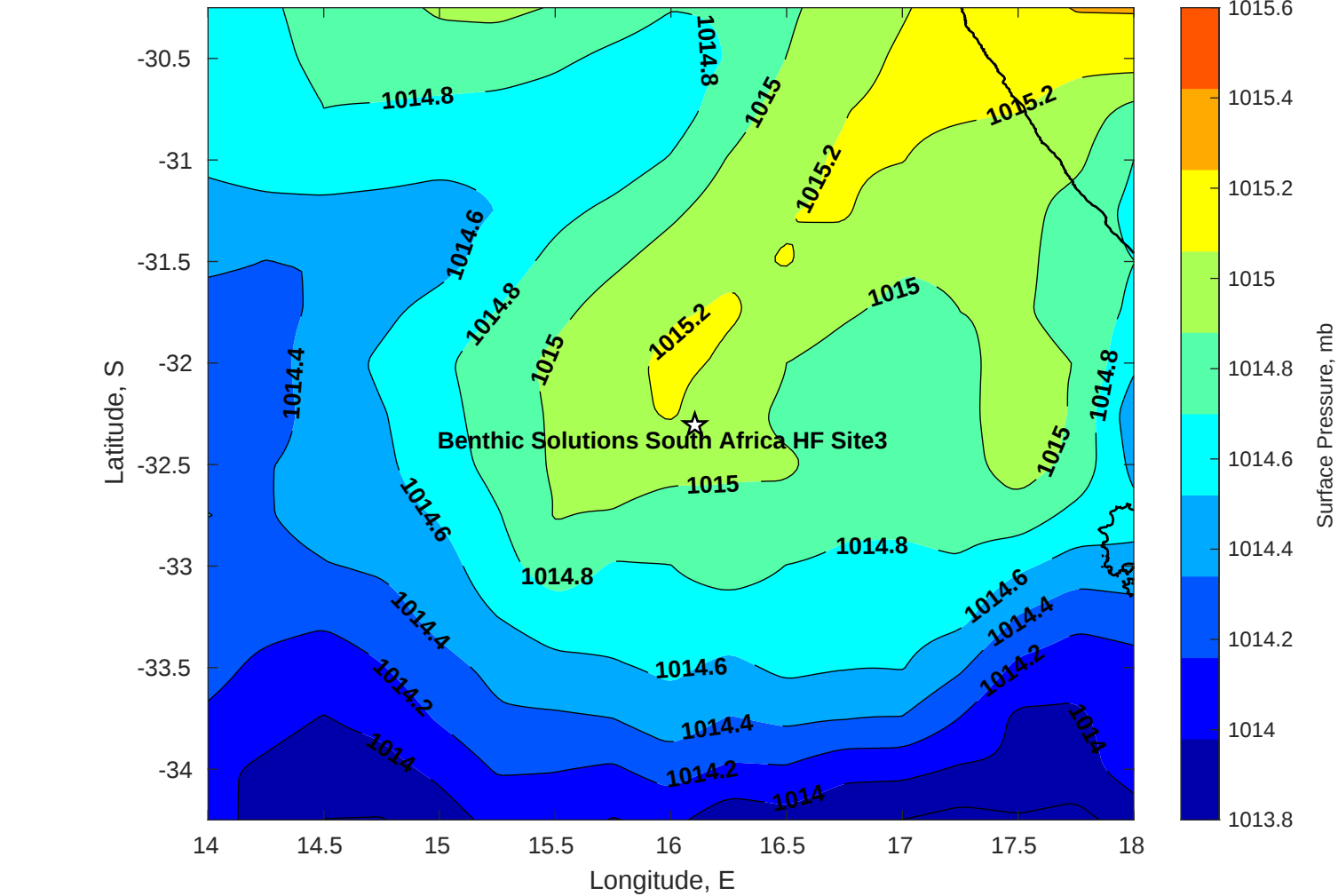
Surface Pressure (mb) for Benthic Solutions South Africa HF Site3 at 08-Apr-2025 00:00:00
