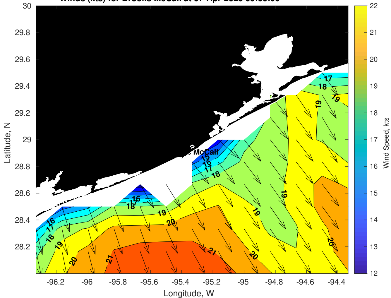
Winds (kts) for Brooks McCall at 07-Apr-2025 09:00:00
