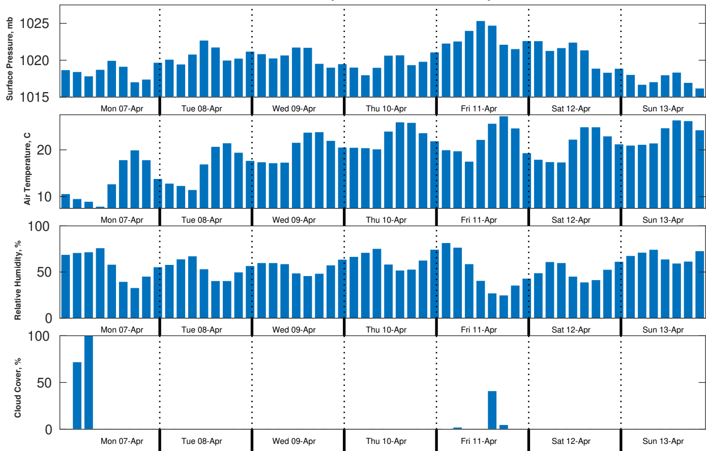
Met Forecast for Brooks McCall from 07-Apr-2025 00:00:00 to 14-Apr-2025 00:00:00
