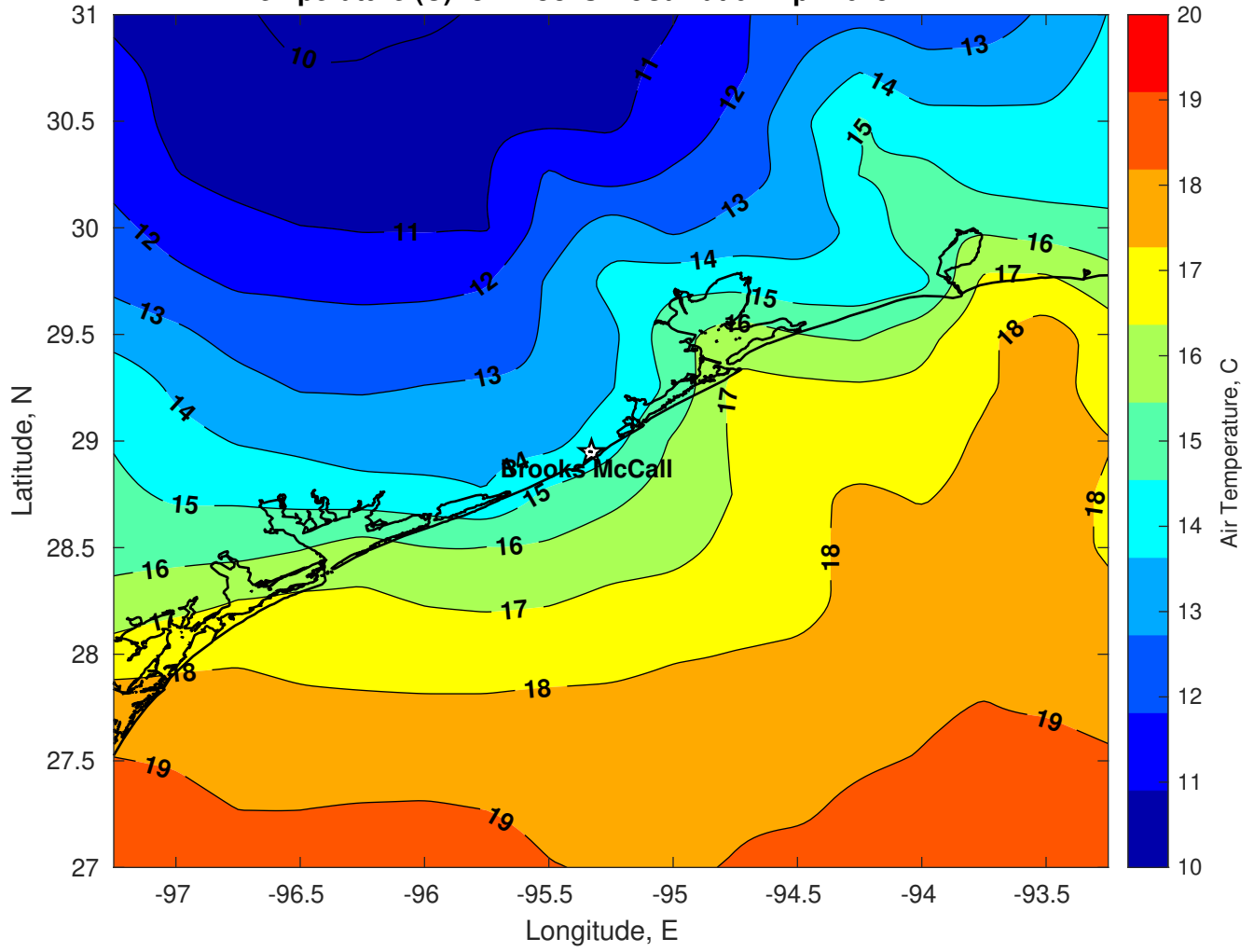
Air Temperature (C) for Brooks McCall at 07-Apr-2025
