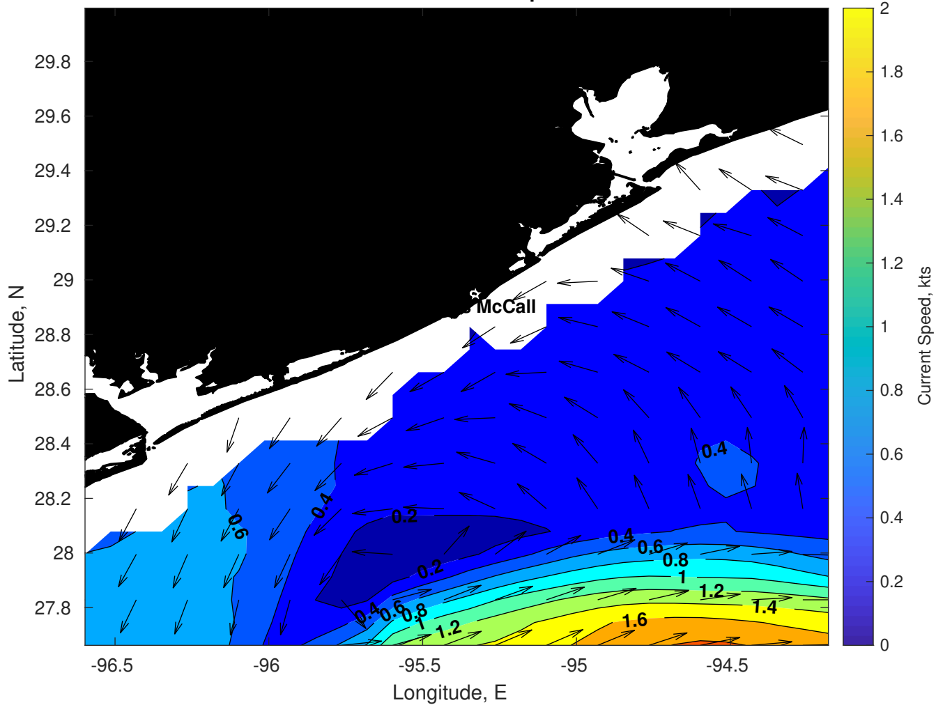
Surface Currents for Brooks McCall at 06-Apr-2025 00:00:00
