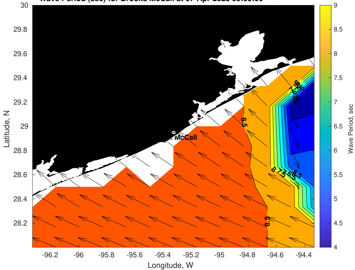
Wave Period (sec) for Brooks McCall at 07-Apr-2025 09:00:00
