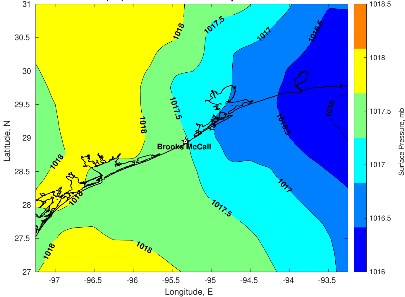
Surface Pressure (mb) for Brooks McCall at 08-Apr-2025 00:00:00
