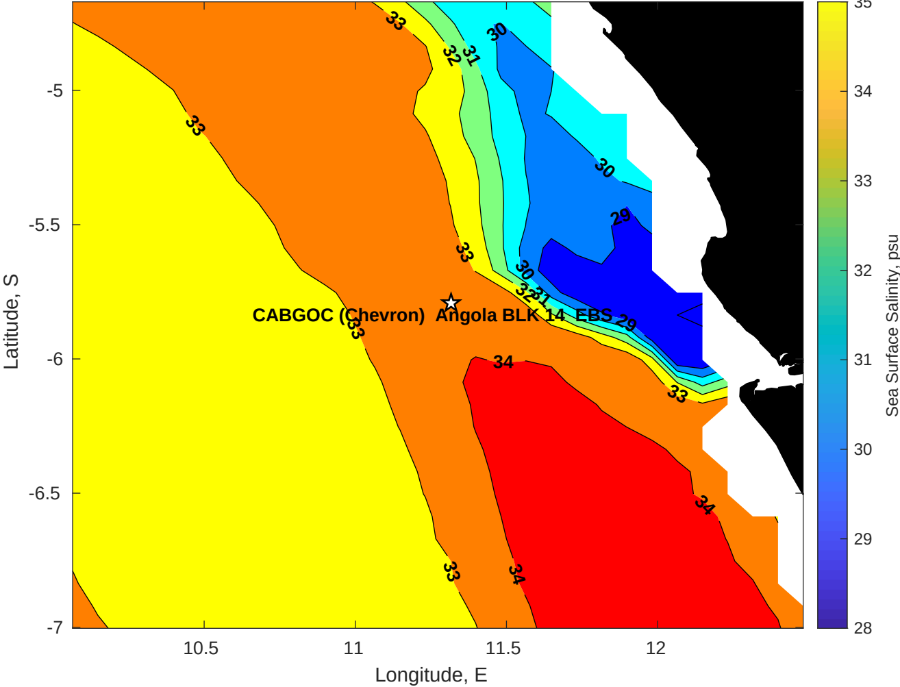
Surface Salinity for CABGOC (Chevron) Angola BLK 14 EBS at 06-Apr-2025 00:00:00
