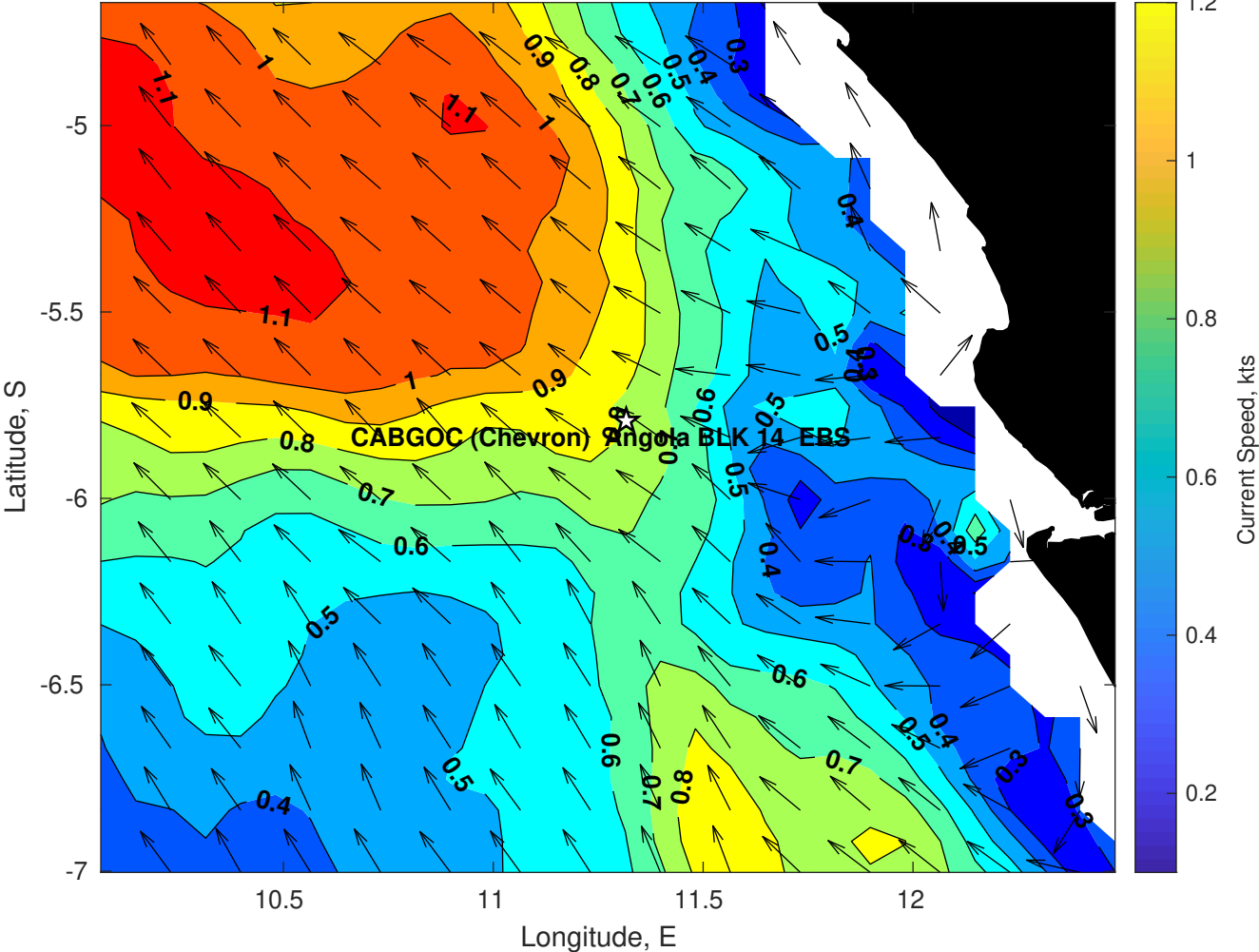
Surface Currents for CABGOC (Chevron) Angola BLK 14 EBS at 06-Apr-2025 00:00:00
