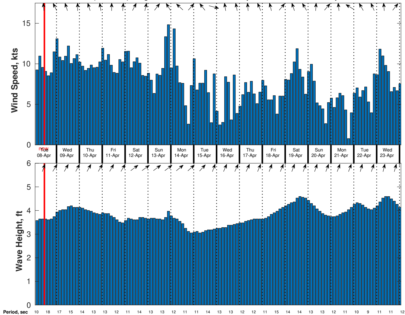
Wind & Wave Forecast for CABGOC (Chevron) Angola BLK 14 EBS from 07-Apr-2025 02:00:00 to 23-Apr-2025 02:00:00
