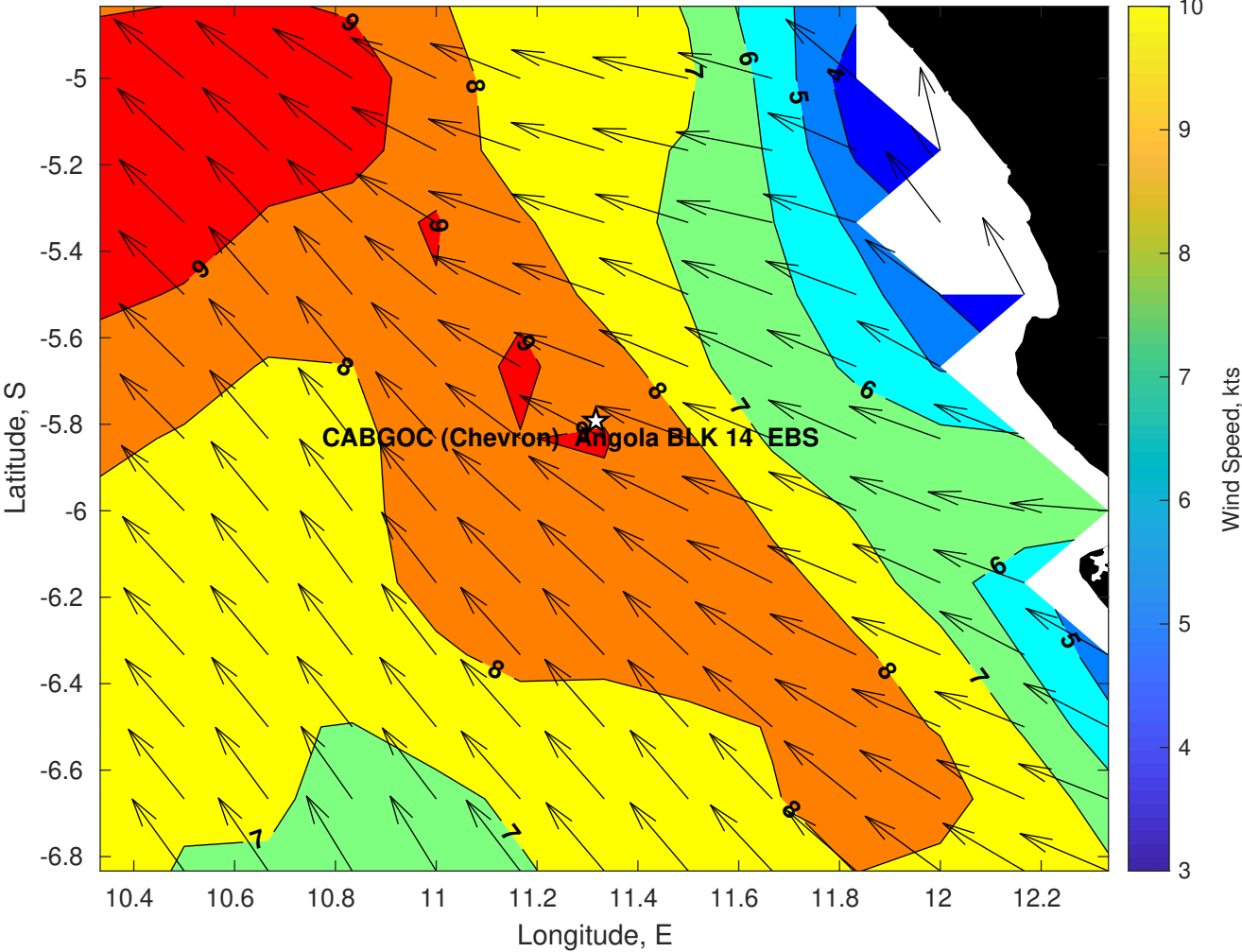
Winds (kts) for CABGOC (Chevron) Angola BLK 14 EBS at 07-Apr-2025 09:00:00
