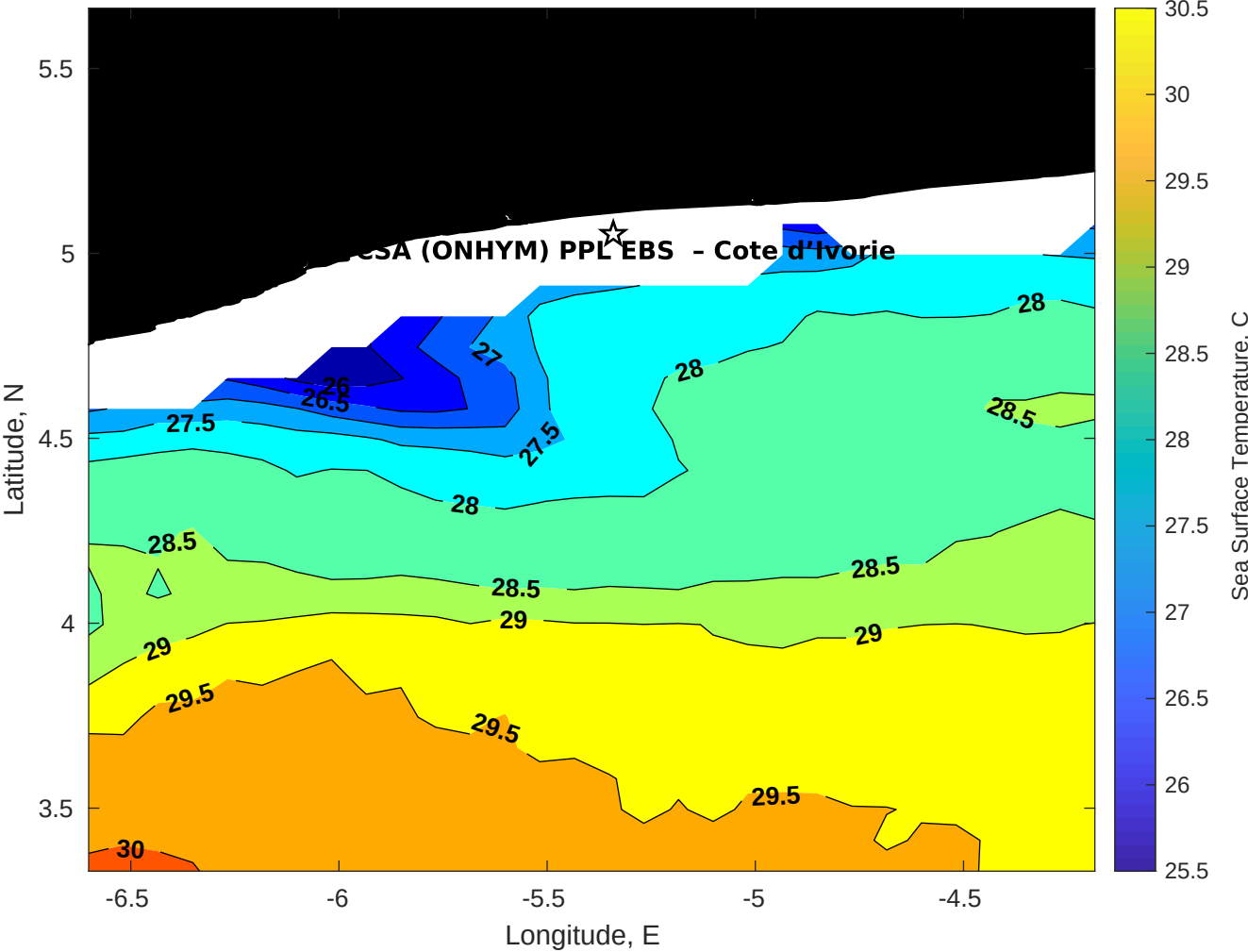
SST for CSA (ONHYM) PPL EBS - Cote d'Ivoire at 06-Apr-2025 00:00:00
