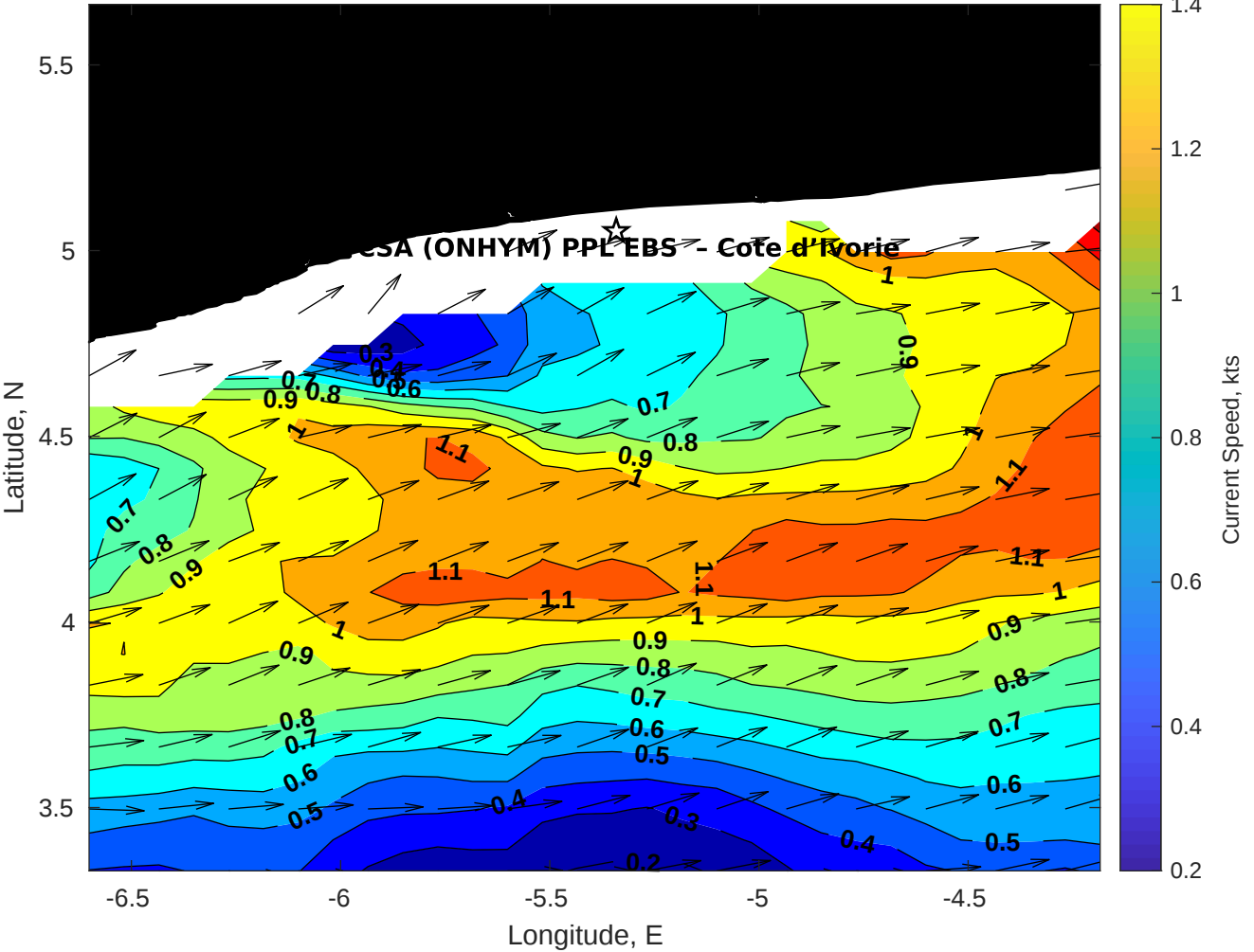
Surface Currents for CSA (ONHYM) PPL EBS - Cote d'Ivoire at 06-Apr-2025 00:00:00
