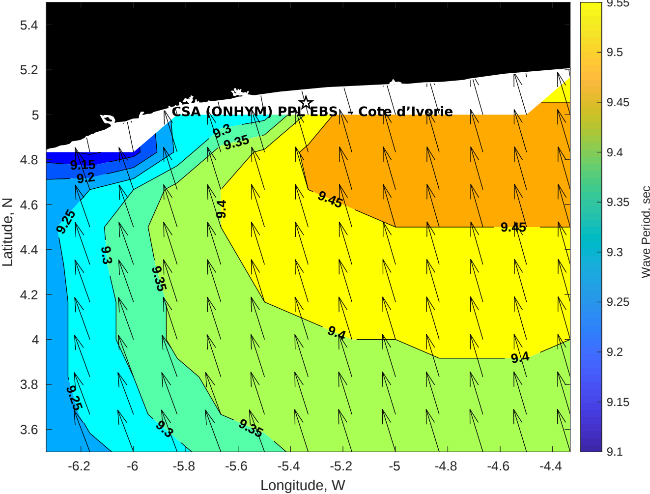
Wave Period (sec) for CSA (ONHYM) PPL EBS - Cote d'Ivoire at 07-Apr-2025 09:00:00
