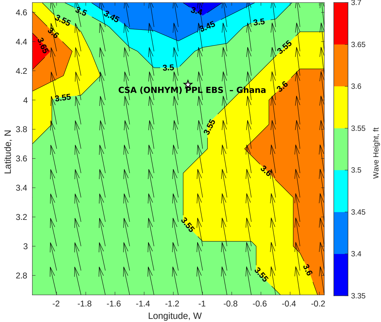
Wave Height (ft) for CSA (ONHYM) PPL EBS - Ghana at 07-Apr-2025 09:00:00
