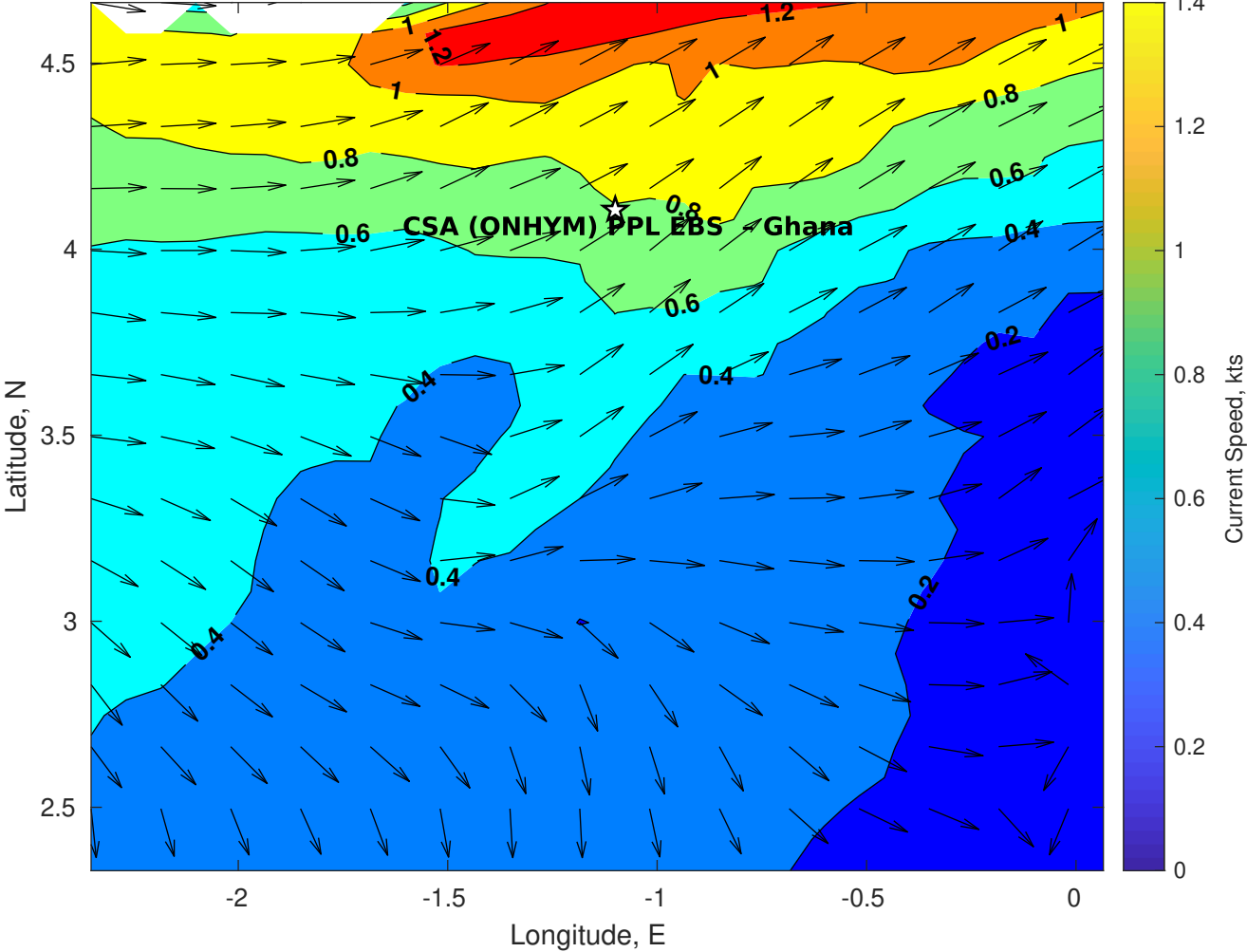
Surface Currents for CSA (ONHYM) PPL EBS - Ghana at 06-Apr-2025 00:00:00
