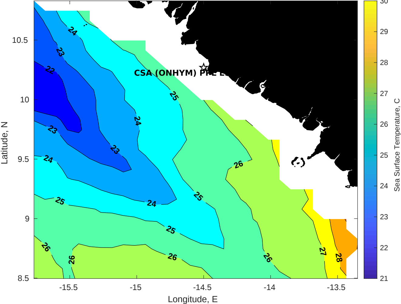
SST for CSA (ONHYM) PPL EBS - Guinea at 06-Apr-2025 00:00:00
