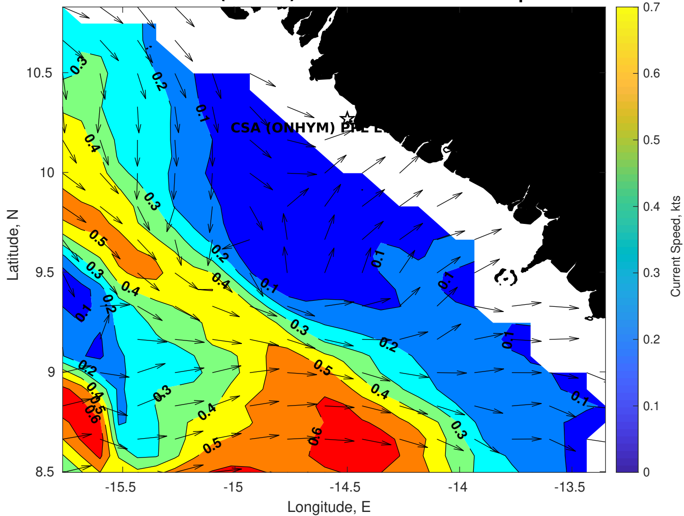
Surface Currents for CSA (ONHYM) PPL EBS - Guinea at 06-Apr-2025 00:00:00
