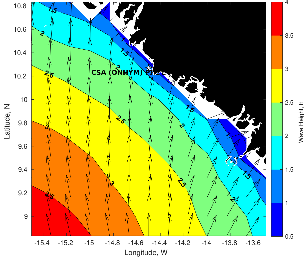
Wave Height (ft) for CSA (ONHYM) PPL EBS - Guinea at 07-Apr-2025 09:00:00
