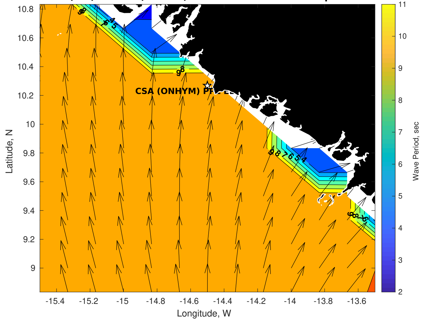
Wave Period (sec) for CSA (ONHYM) PPL EBS - Guinea at 07-Apr-2025 09:00:00
