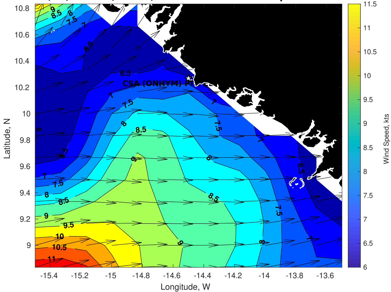
Winds (kts) for CSA (ONHYM) PPL EBS - Guinea at 07-Apr-2025 09:00:00
