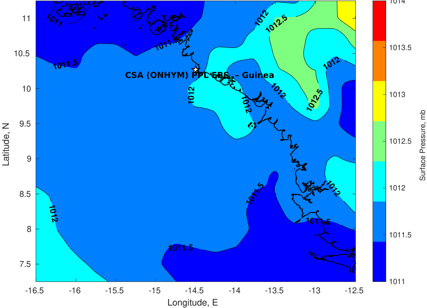
Surface Pressure (mb) for CSA (ONHYM) PPL EBS - Guinea at 08-Apr-2025 00:00:00
