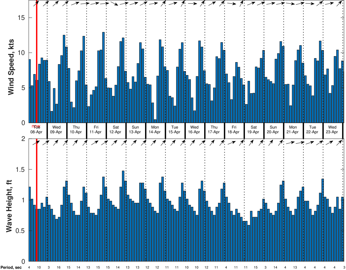
Wind & Wave Forecast for CSA (ONHYM) PPL EBS - Guinea from 07-Apr-2025 01:00:00 to 23-Apr-2025 01:00:00
