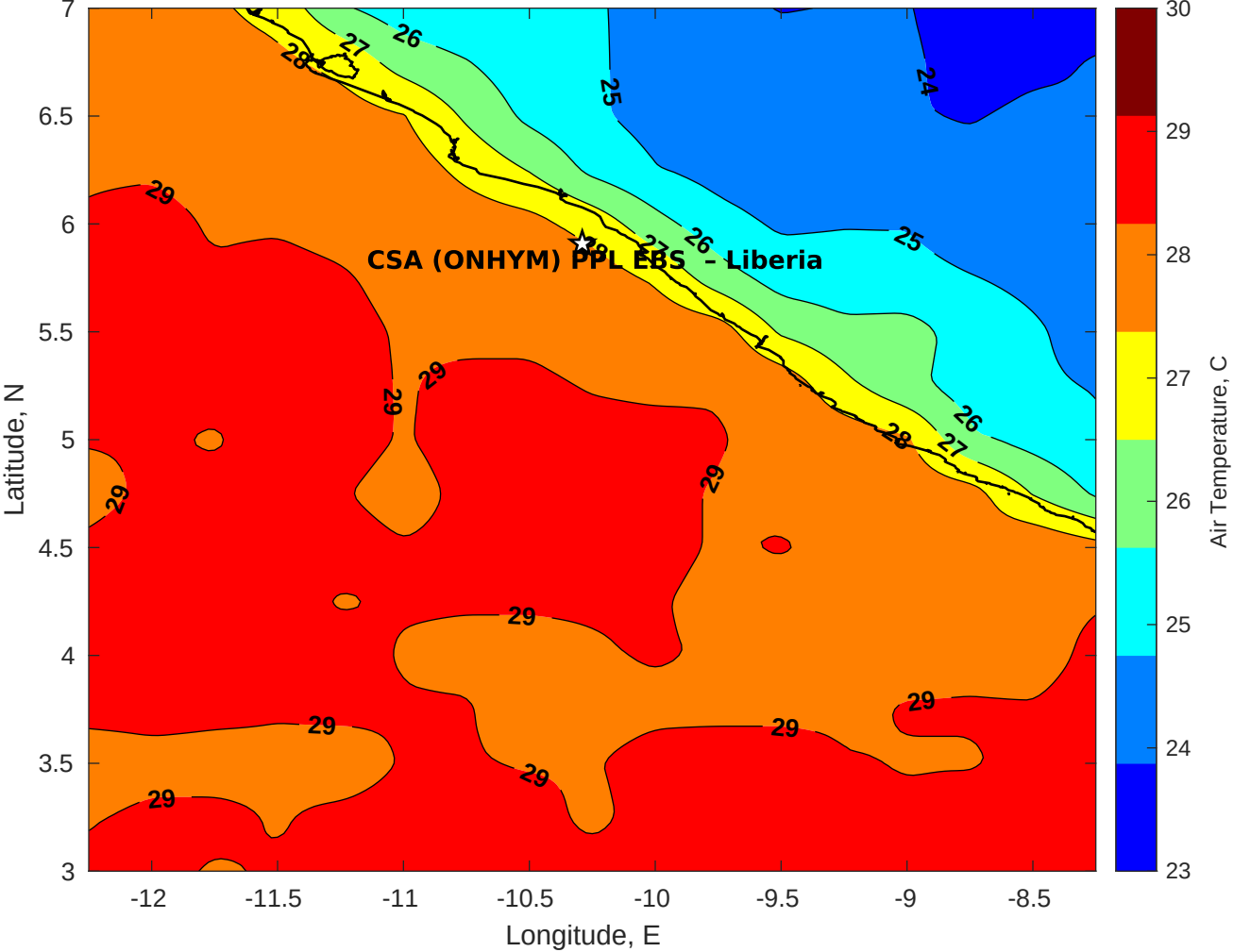
Air Temperature (C) for CSA (ONHYM) PPL EBS - Liberia at 07-Apr-2025
