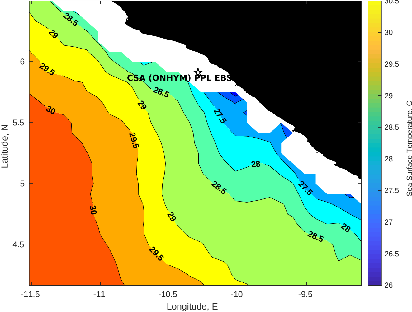
SST for CSA (ONHYM) PPL EBS - Liberia at 06-Apr-2025 00:00:00
