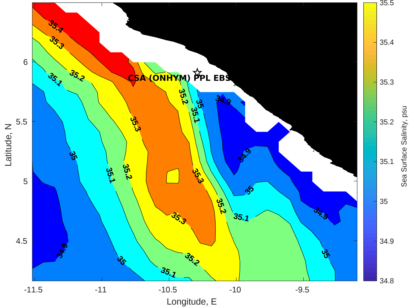
Surface Salinity for CSA (ONHYM) PPL EBS - Liberia at 06-Apr-2025 00:00:00
