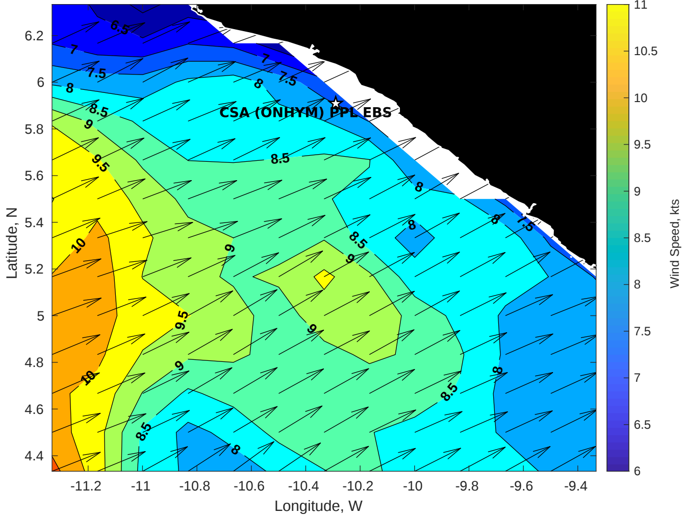
Winds (kts) for CSA (ONHYM) PPL EBS - Liberia at 07-Apr-2025 09:00:00
