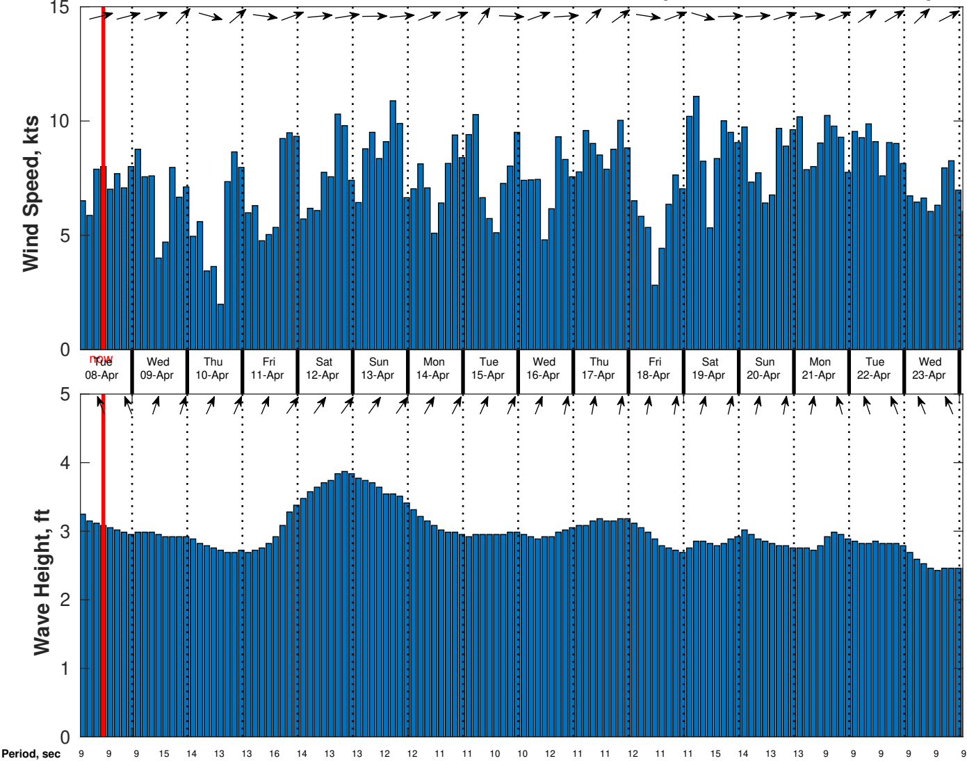
Wind & Wave Forecast for CSA (ONHYM) PPL EBS - Liberia from 07-Apr-2025 01:00:00 to 23-Apr-2025 01:00:00
