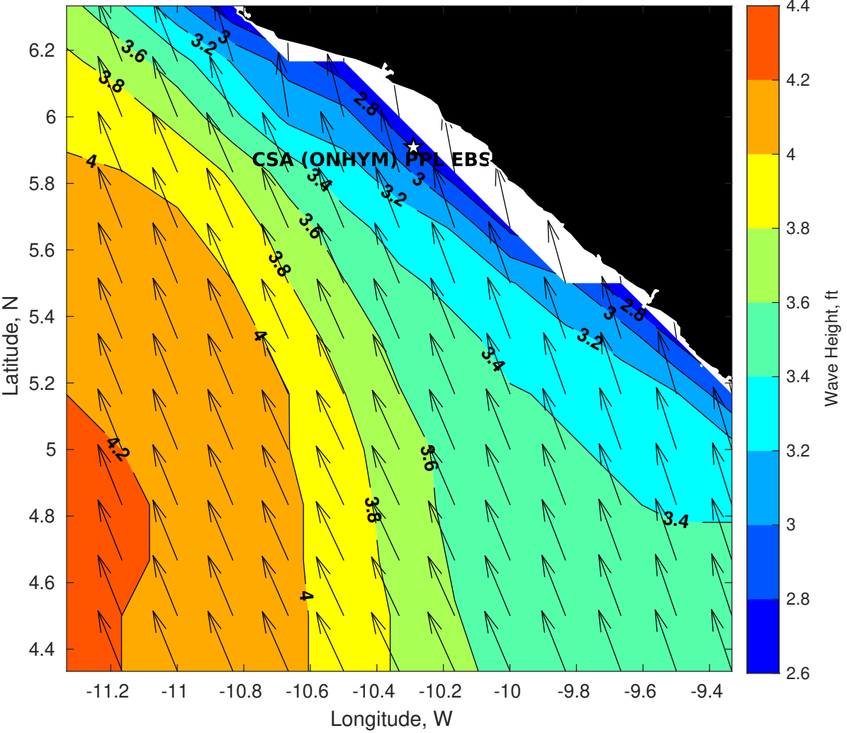
Wave Height (ft) for CSA (ONHYM) PPL EBS - Liberia at 07-Apr-2025 09:00:00
