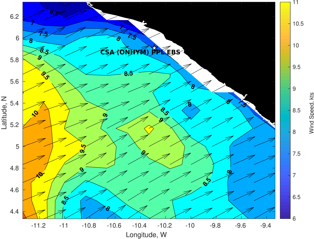
Winds (kts) for CSA (ONHYM) PPL EBS - Liberia at 07-Apr-2025 09:00:00
