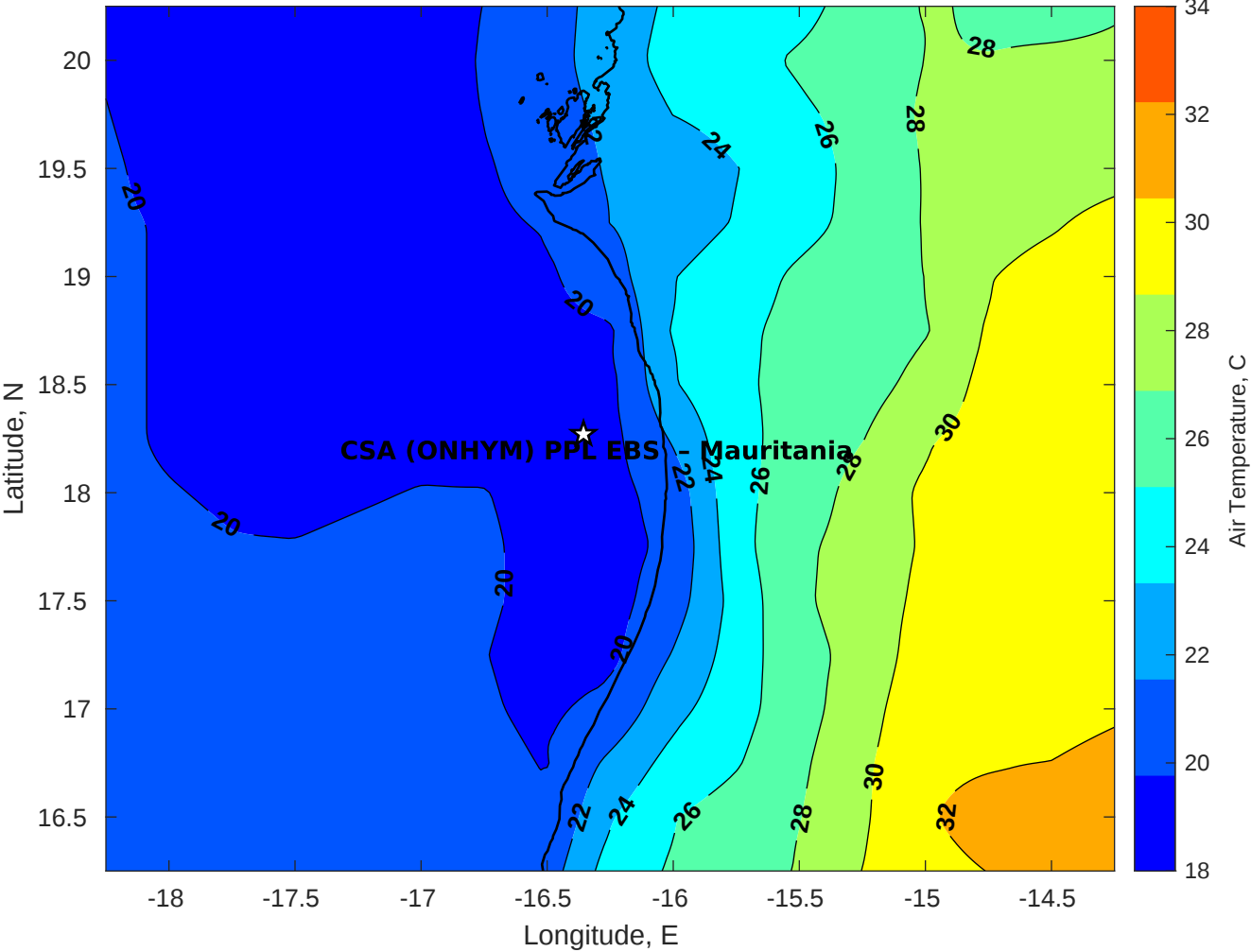
Air Temperature (C) for CSA (ONHYM) PPL EBS - Mauritania at 07-Apr-2025
