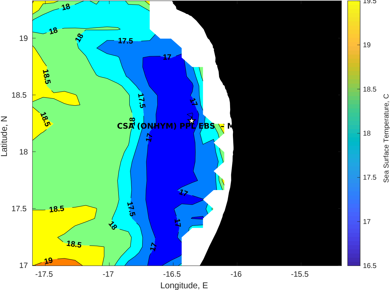
SST for CSA (ONHYM) PPL EBS - Mauritania at 06-Apr-2025 00:00:00
