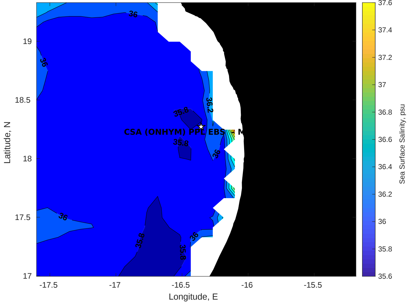
Surface Salinity for CSA (ONHYM) PPL EBS - Mauritania at 06-Apr-2025 00:00:00
