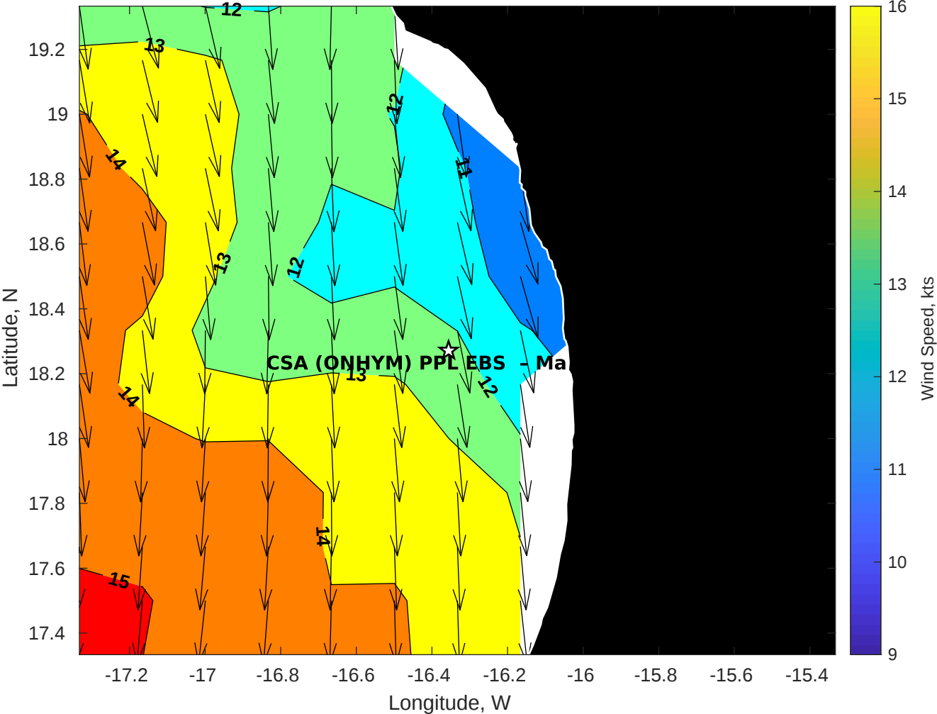
Winds (kts) for CSA (ONHYM) PPL EBS - Mauritania at 07-Apr-2025 09:00:00
