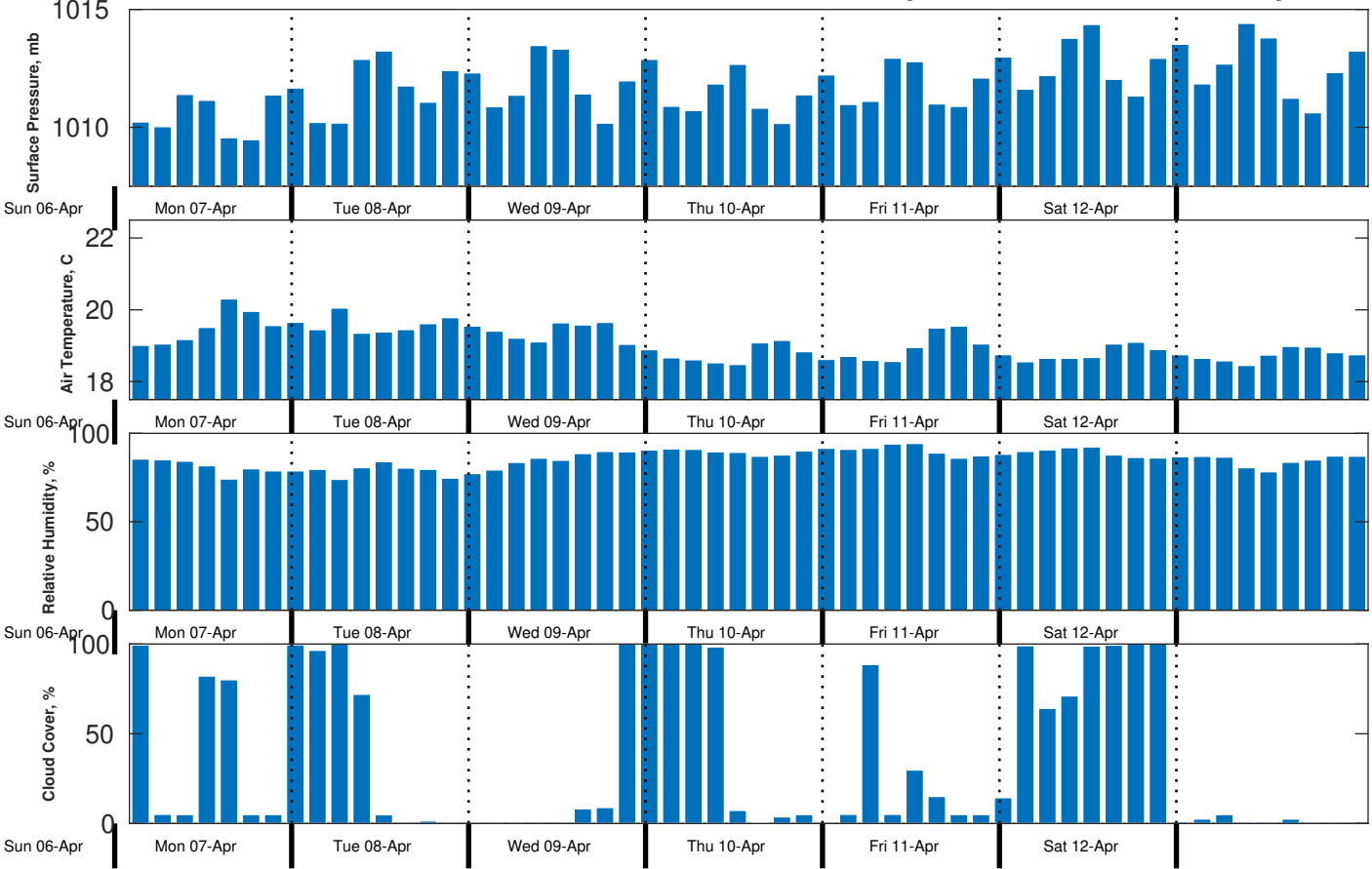
Met Forecast for CSA (ONHYM) PPL EBS - Mauritania from 07-Apr-2025 00:00:00 to 14-Apr-2025 00:00:00
