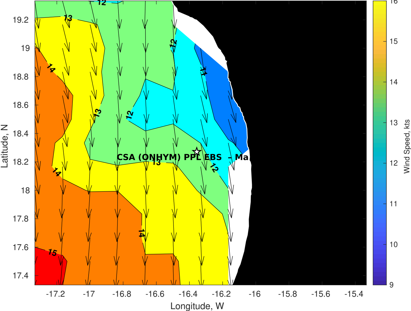
Winds (kts) for CSA (ONHYM) PPL EBS - Mauritania at 07-Apr-2025 09:00:00
