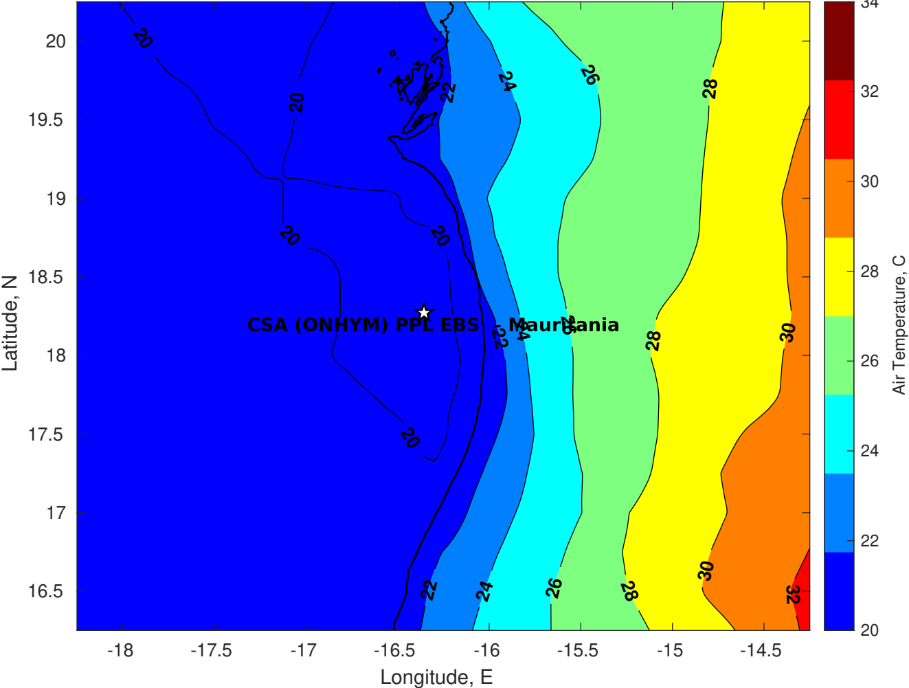
Air Temperature (C) for CSA (ONHYM) PPL EBS - Mauritania at 07-Apr-2025
