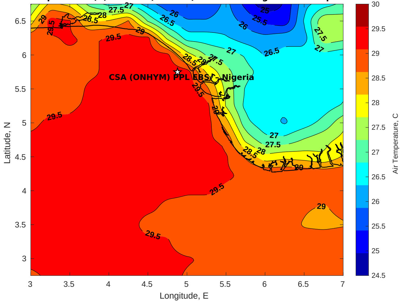
Air Temperature (C) for CSA (ONHYM) PPL EBS - Nigeria at 07-Apr-2025
