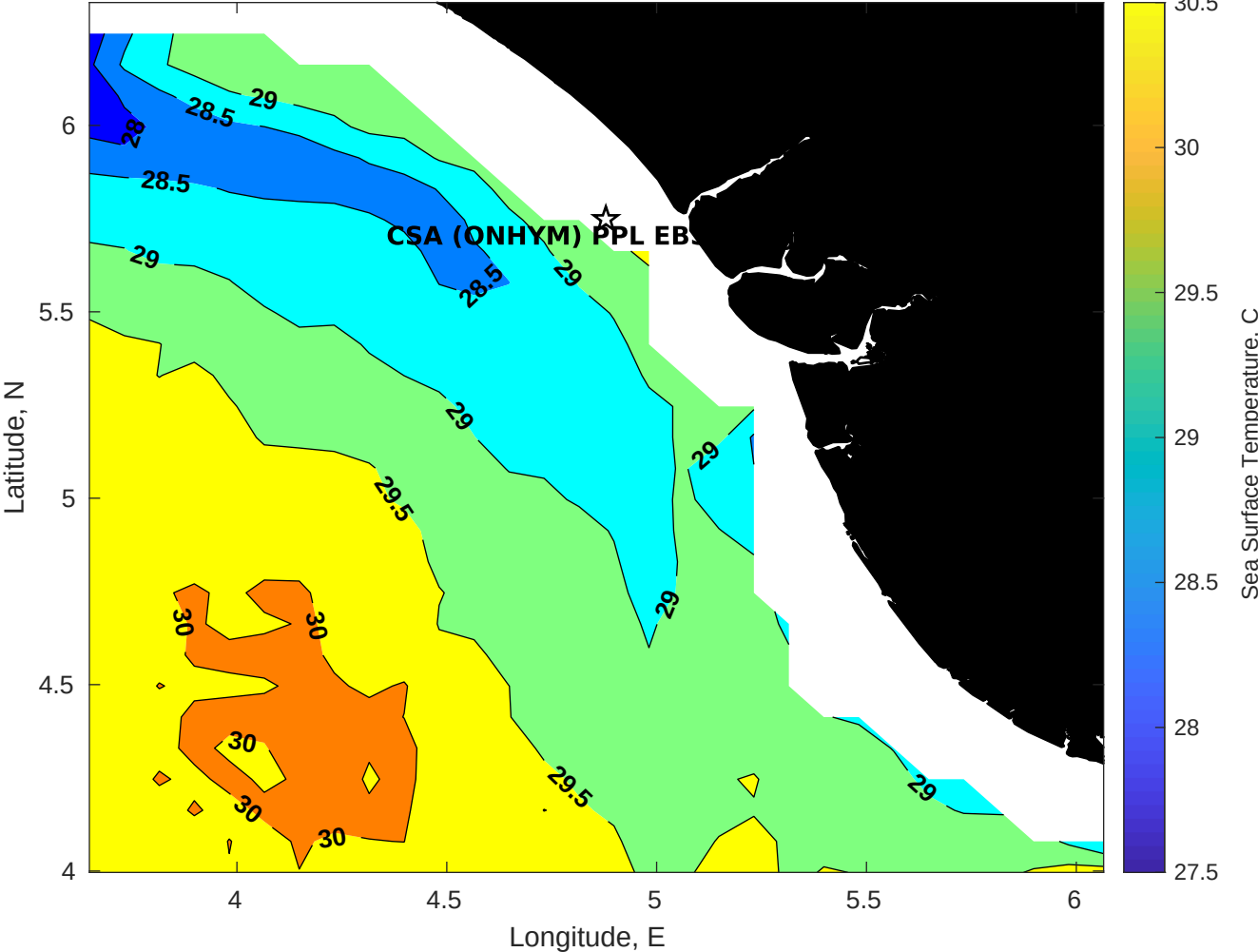
SST for CSA (ONHYM) PPL EBS - Nigeria at 06-Apr-2025 00:00:00
