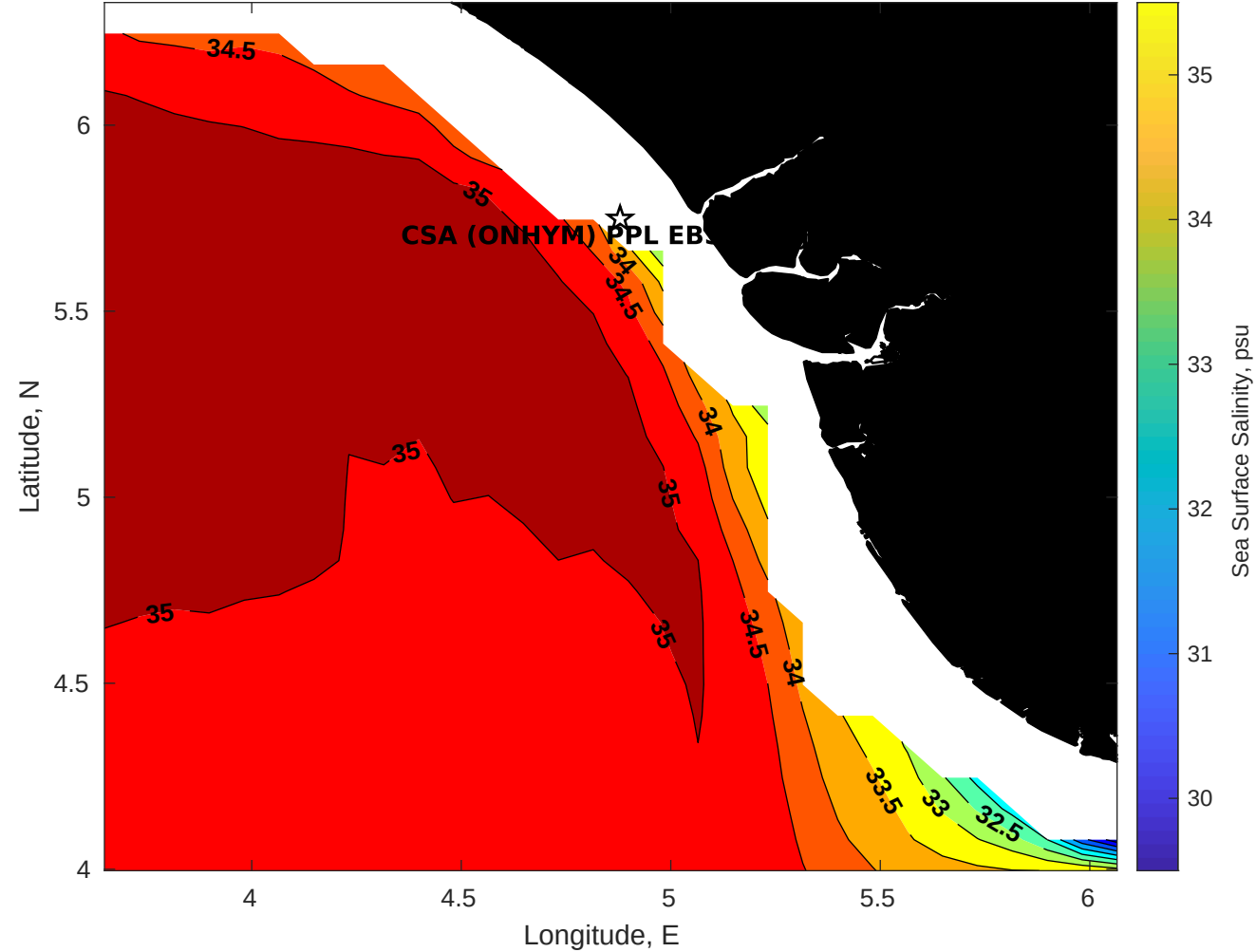
Surface Salinity for CSA (ONHYM) PPL EBS - Nigeria at 06-Apr-2025 00:00:00
