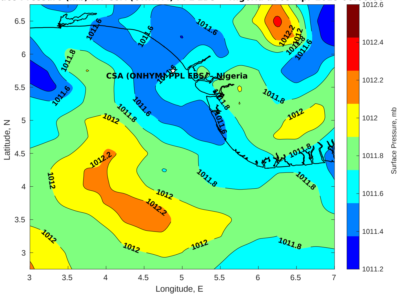
Surface Pressure (mb) for CSA (ONHYM) PPL EBS - Nigeria at 09-Apr-2025 00:00:00
