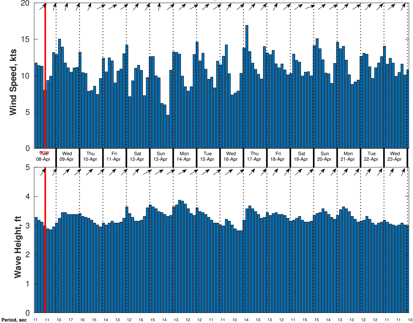
Wind & Wave Forecast for CSA (ONHYM) PPL EBS - Nigeria from 07-Apr-2025 02:00:00 to 23-Apr-2025 02:00:00
