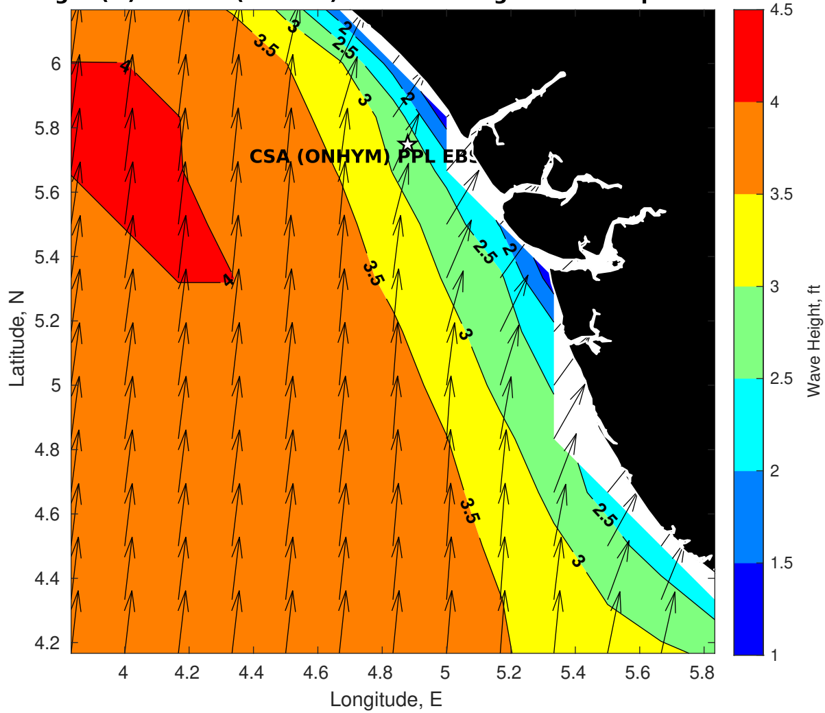
Wave Height (ft) for CSA (ONHYM) PPL EBS - Nigeria at 07-Apr-2025 09:00:00
