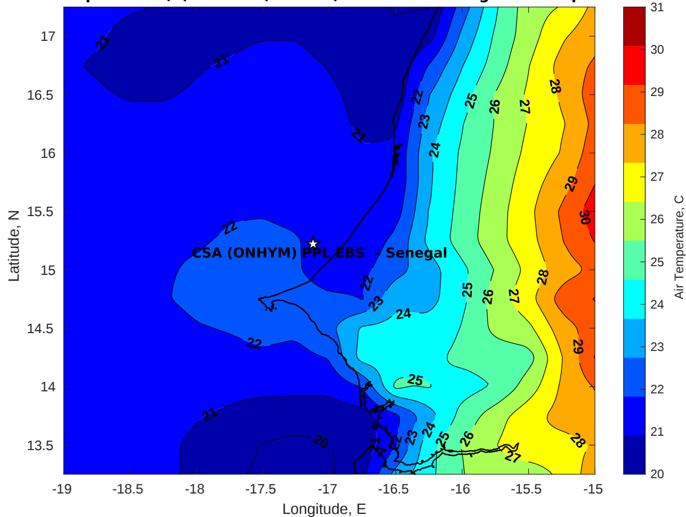
Air Temperature (C) for CSA (ONHYM) PPL EBS - Senegal at 07-Apr-2025
