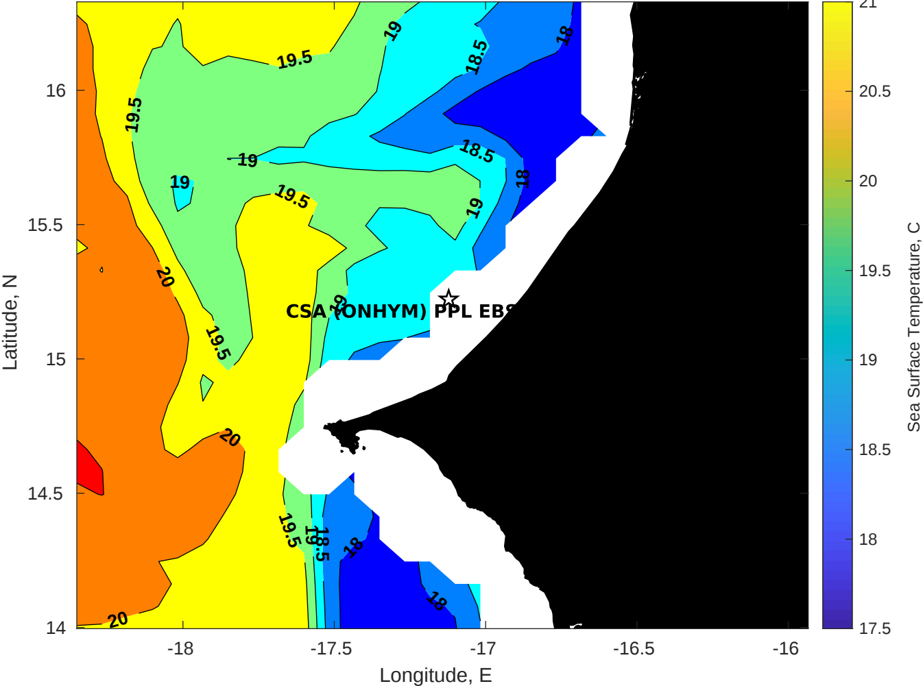
SST for CSA (ONHYM) PPL EBS - Senegal at 06-Apr-2025 00:00:00
