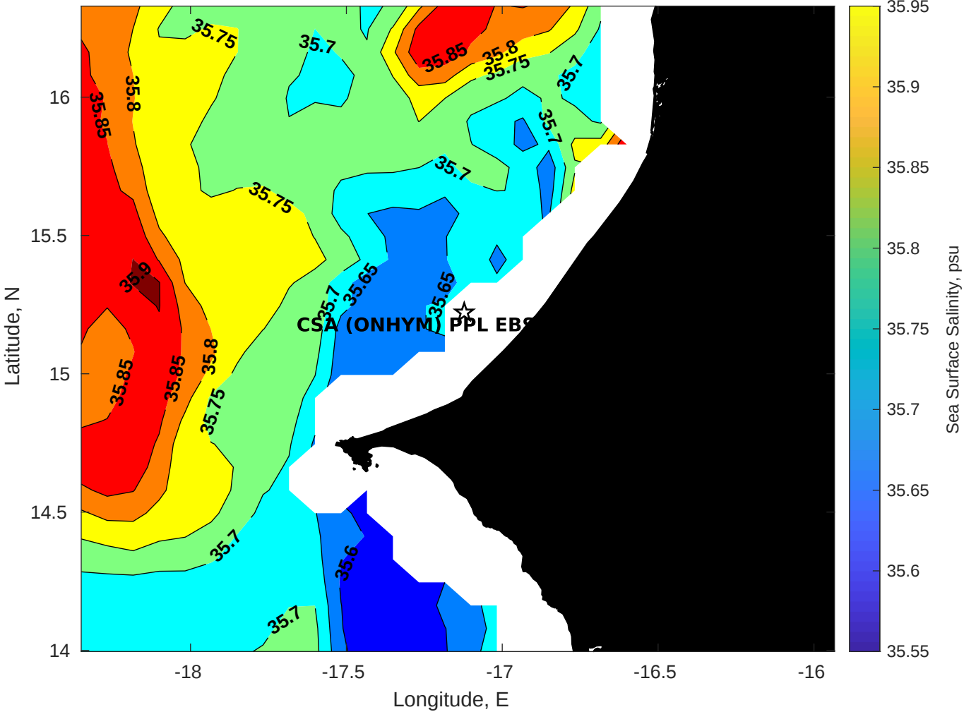
Surface Salinity for CSA (ONHYM) PPL EBS - Senegal at 06-Apr-2025 00:00:00
