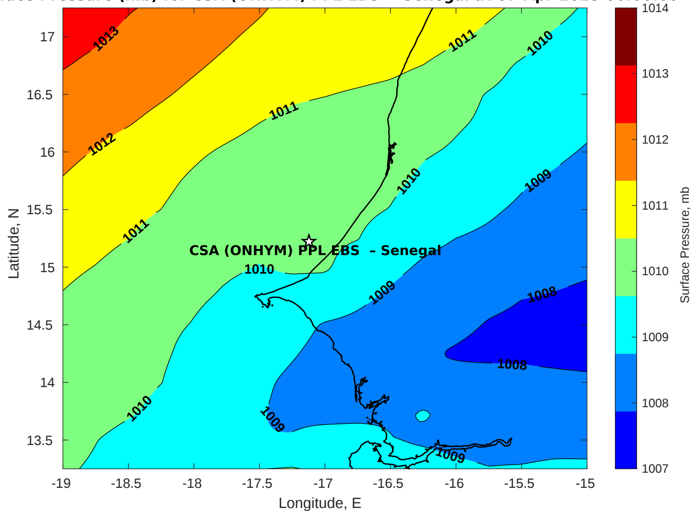
Surface Pressure (mb) for CSA (ONHYM) PPL EBS - Senegal at 07-Apr-2025 00:00:00
