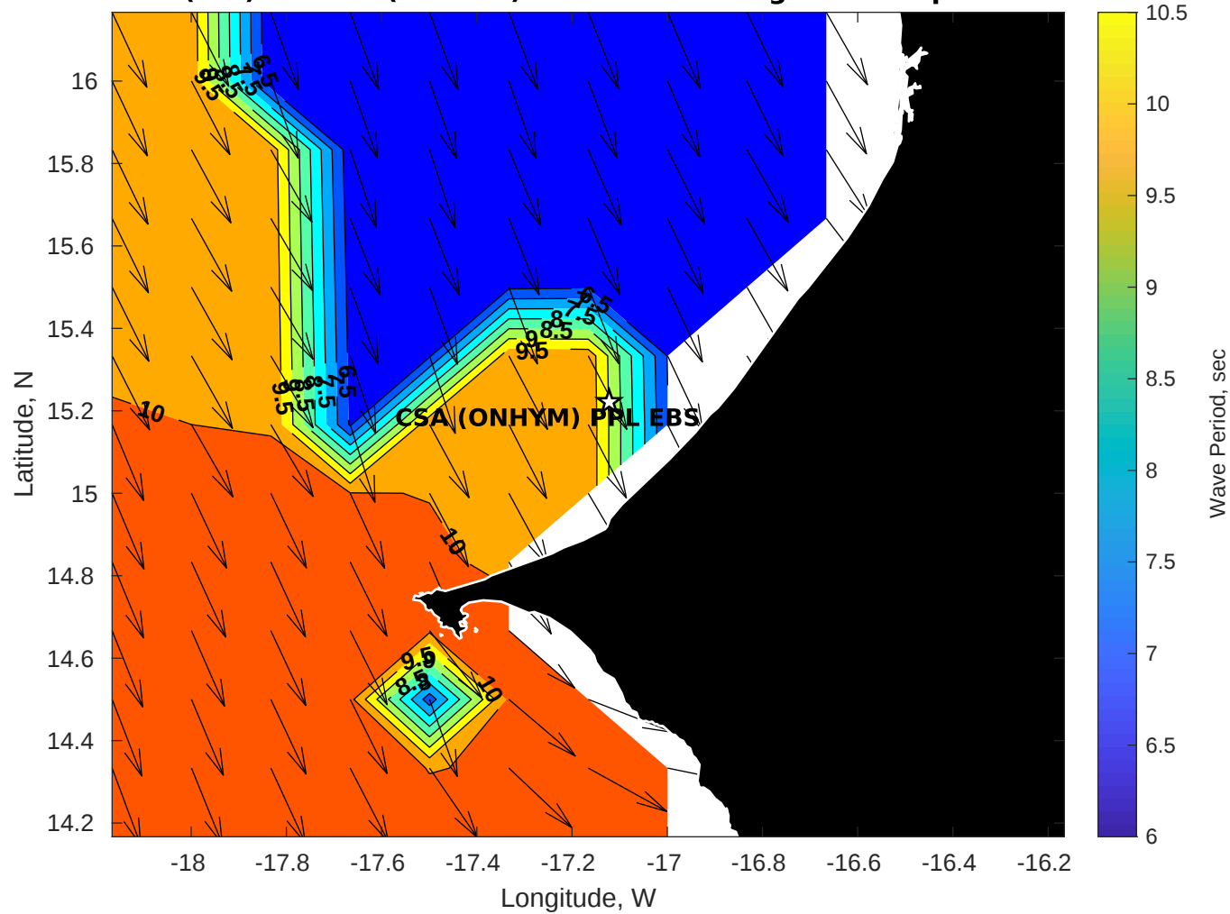
Wave Period (sec) for CSA (ONHYM) PPL EBS - Senegal at 07-Apr-2025 09:00:00
