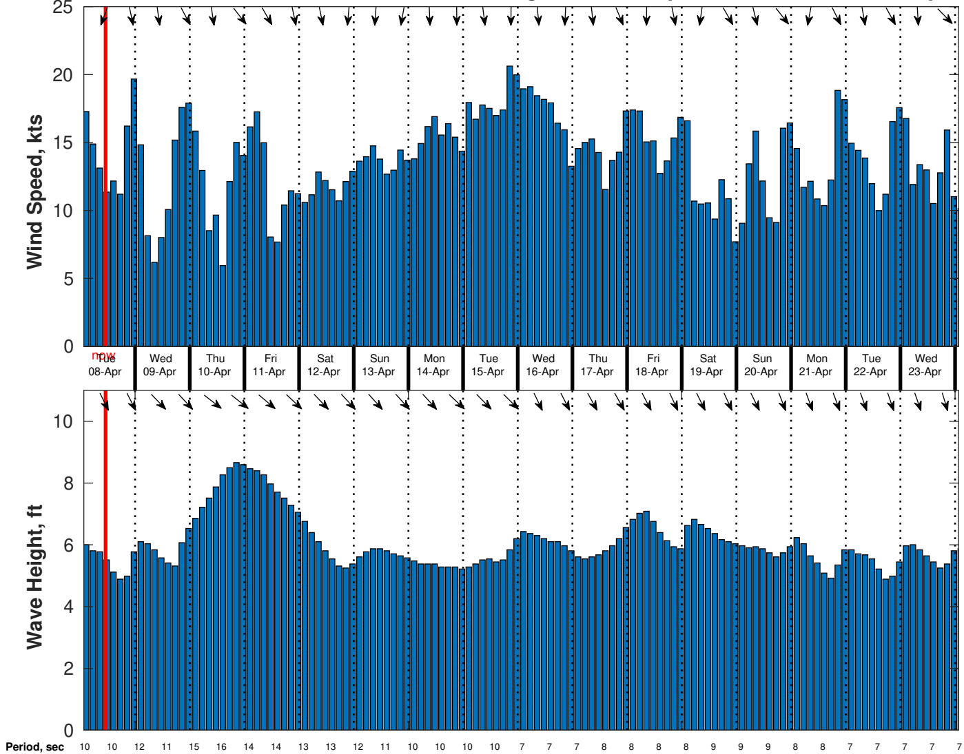
Wind & Wave Forecast for CSA (ONHYM) PPL EBS - Senegal from 07-Apr-2025 01:00:00 to 23-Apr-2025 01:00:00
