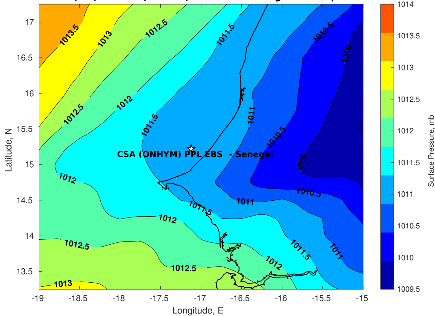
Surface Pressure (mb) for CSA (ONHYM) PPL EBS - Senegal at 09-Apr-2025 00:00:00
