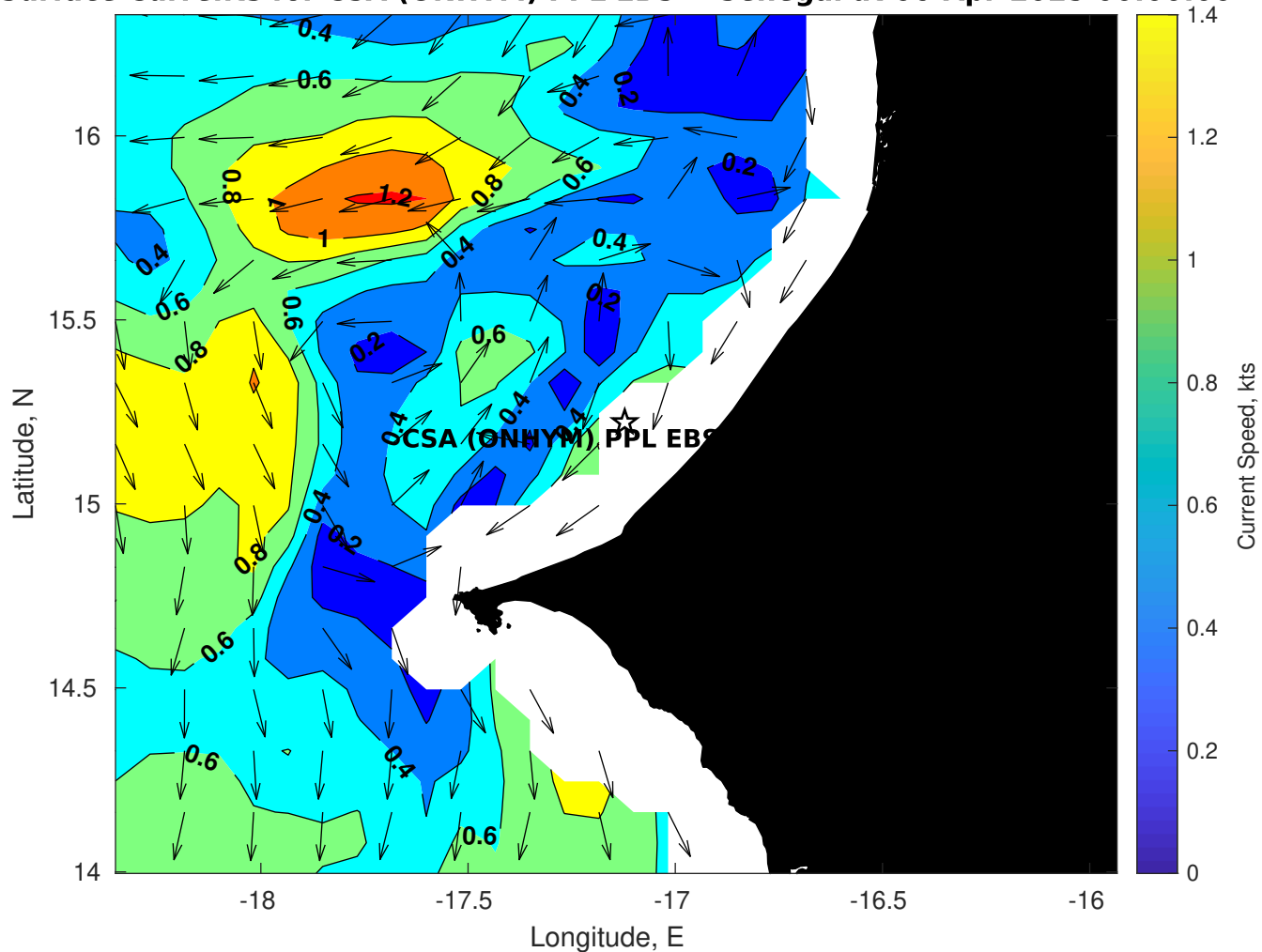
Surface Currents for CSA (ONHYM) PPL EBS - Senegal at 06-Apr-2025 00:00:00
