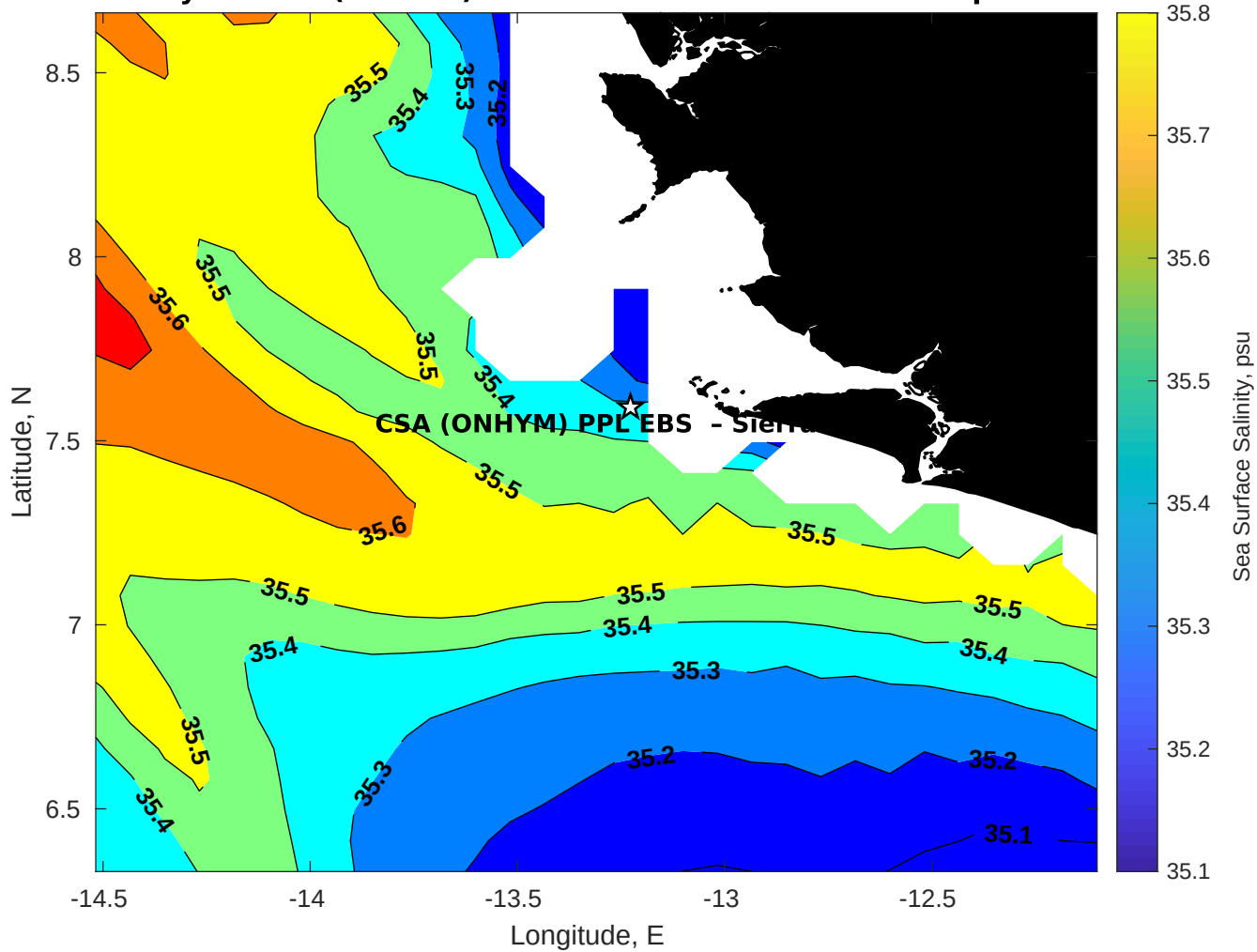
Surface Salinity for CSA (ONHYM) PPL EBS - Sierra Leone at 06-Apr-2025 00:00:00
