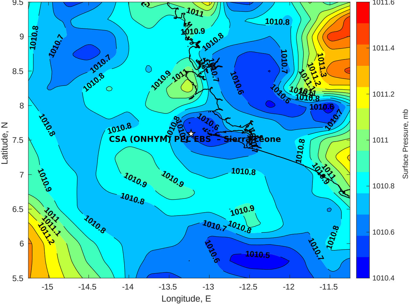
Surface Pressure (mb) for CSA (ONHYM) PPL EBS - Sierra Leone at 07-Apr-2025 00:00:00
