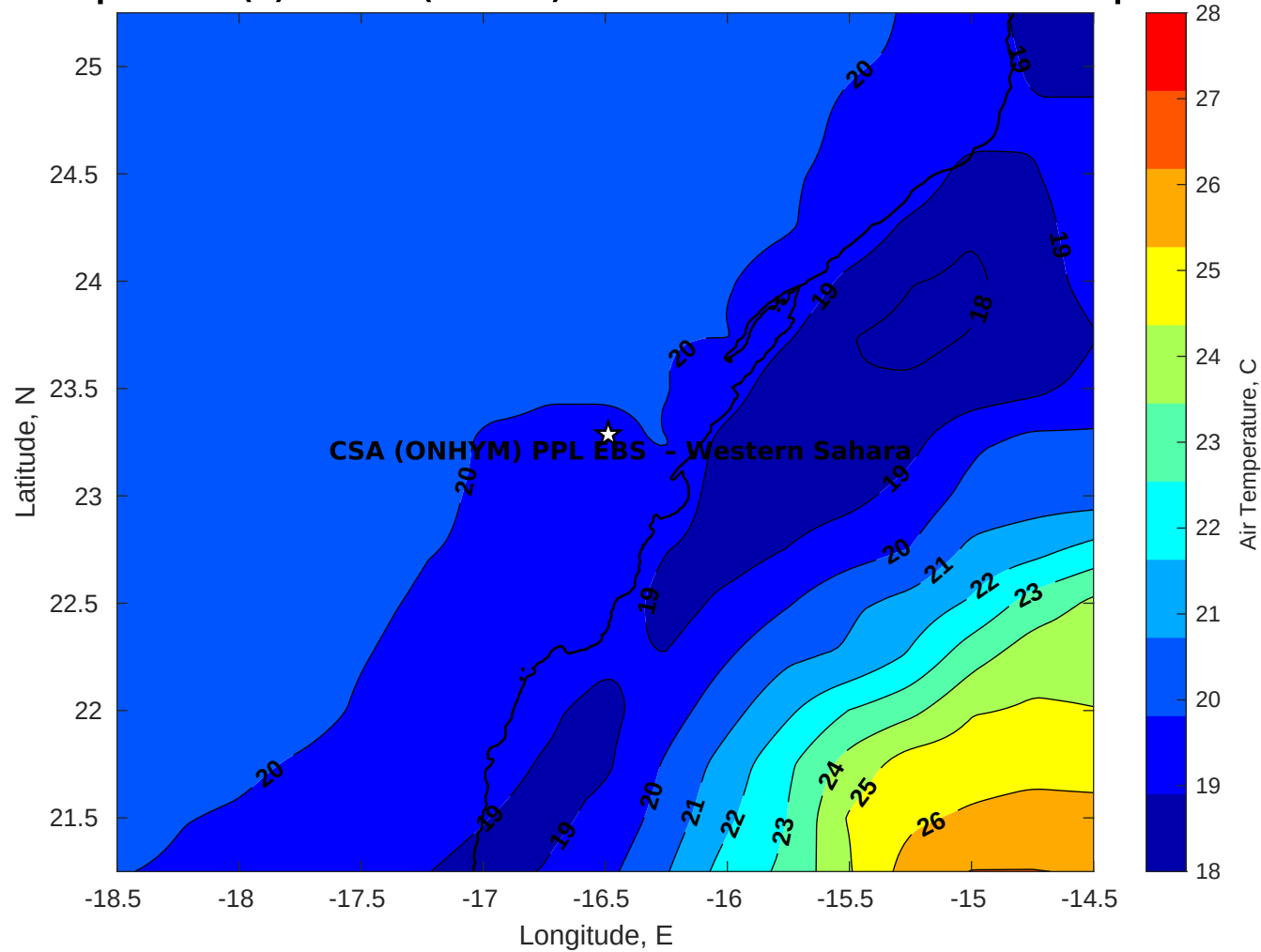
Air Temperature (C) for CSA (ONHYM) PPL EBS - Western Sahara at 07-Apr-2025
