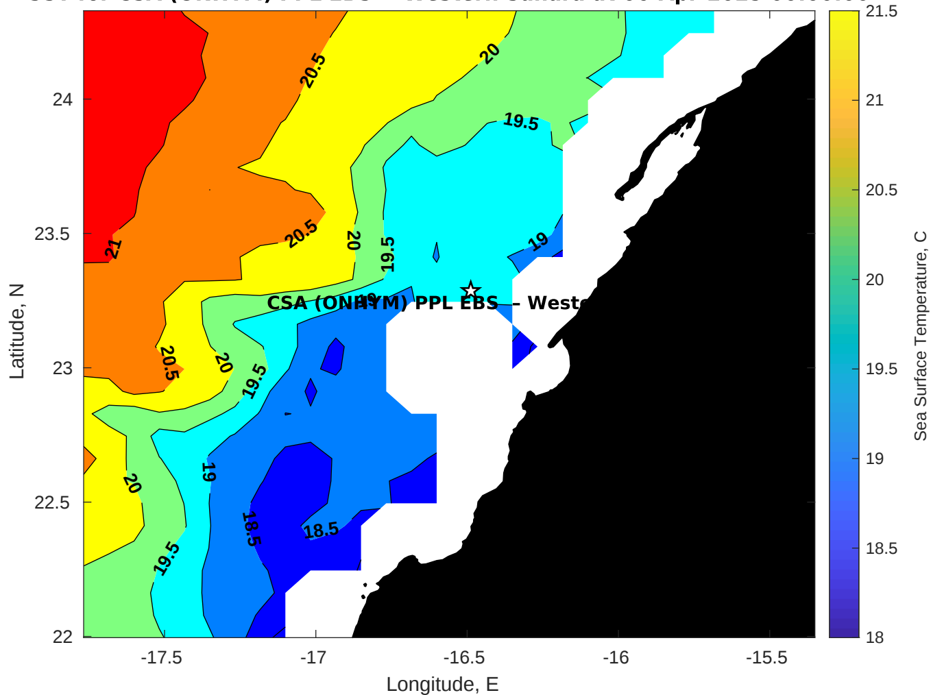
SST for CSA (ONHYM) PPL EBS - Western Sahara at 06-Apr-2025 00:00:00
