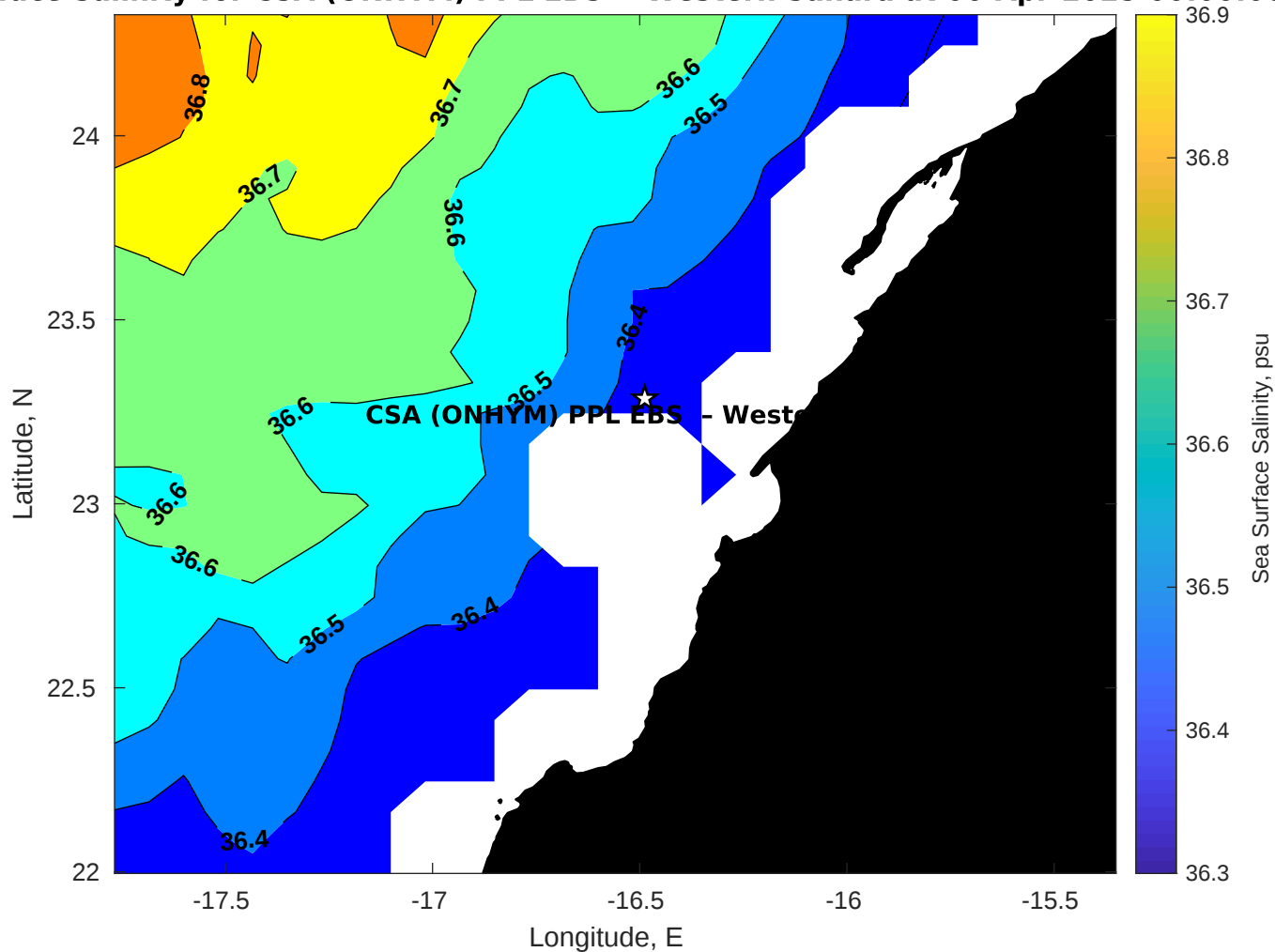
Surface Salinity for CSA (ONHYM) PPL EBS - Western Sahara at 06-Apr-2025 00:00:00
