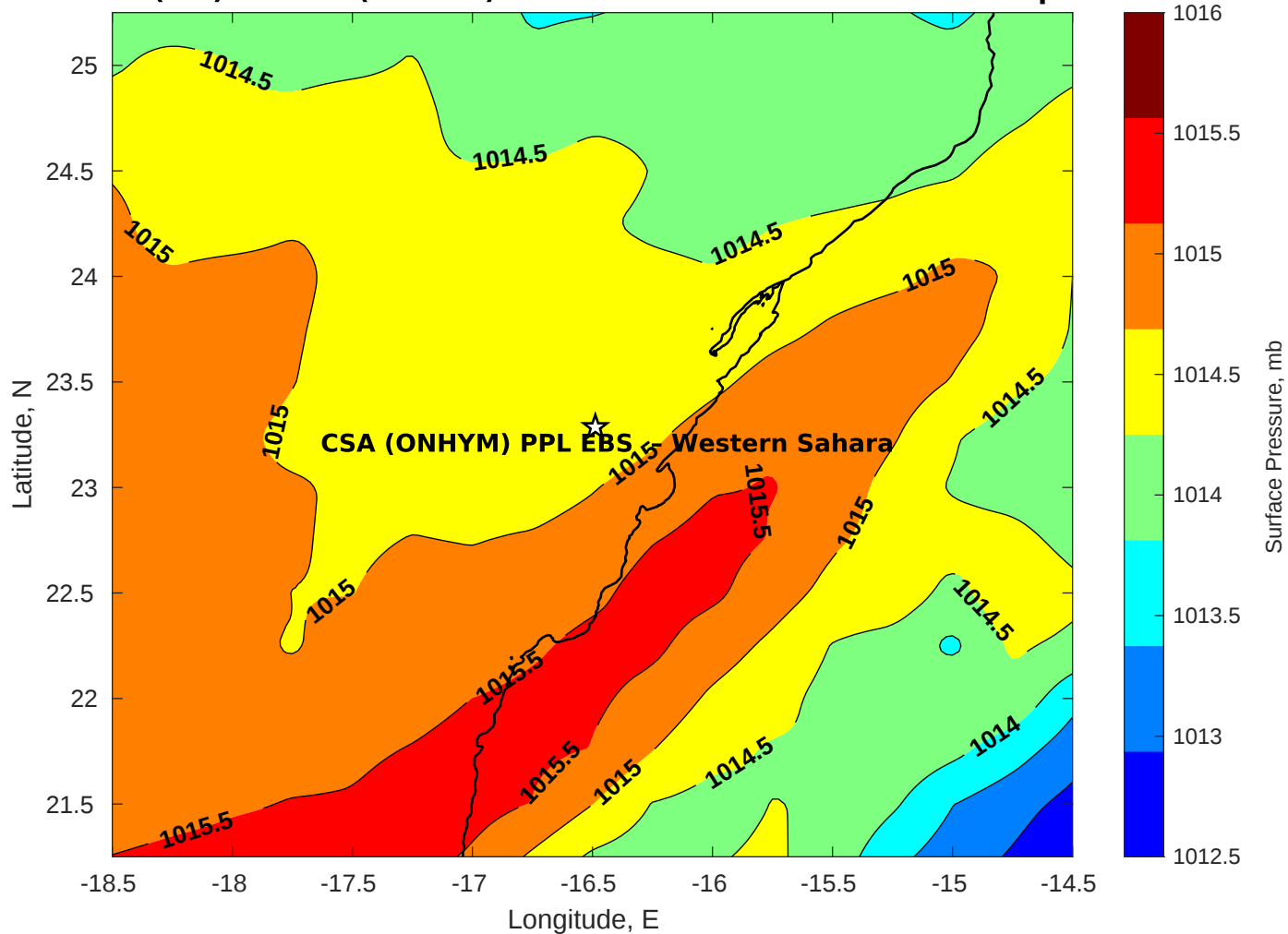
Surface Pressure (mb) for CSA (ONHYM) PPL EBS - Western Sahara at 09-Apr-2025 00:00:00
