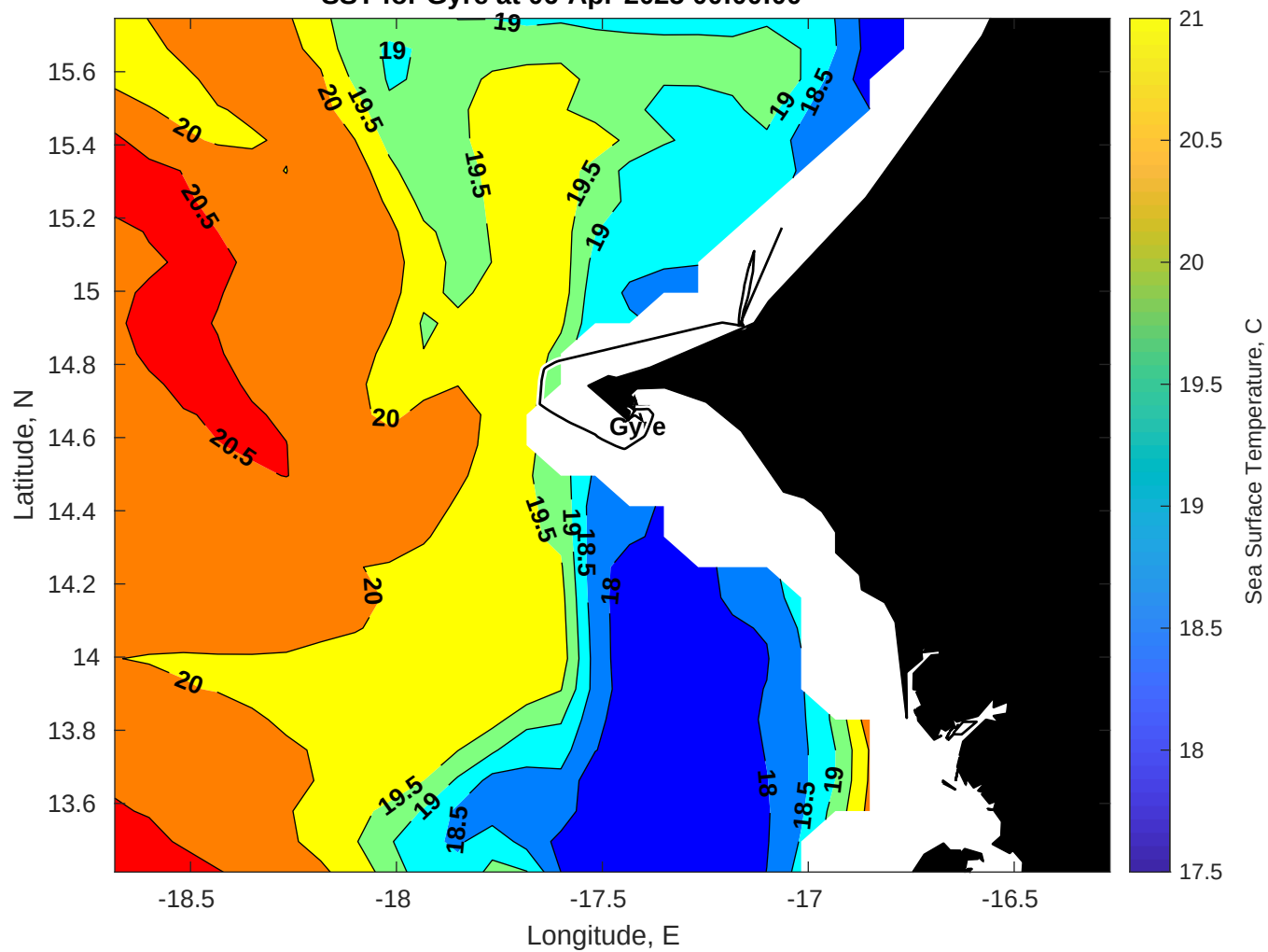
SST for Gyre at 06-Apr-2025 00:00:00
