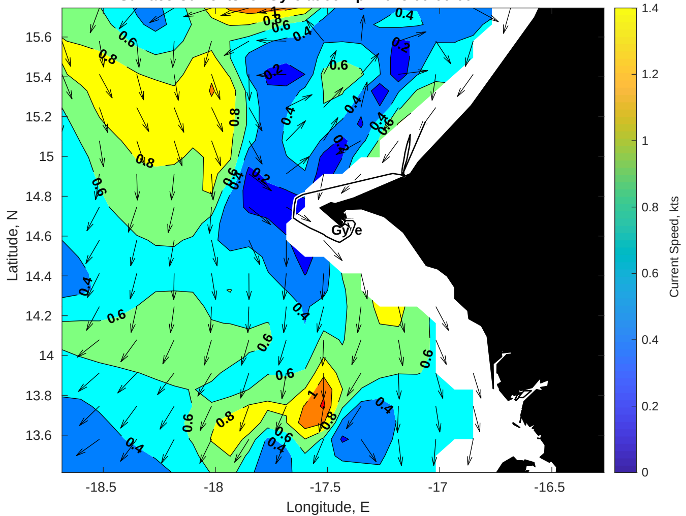
Surface Currents for Gyre at 06-Apr-2025 00:00:00
