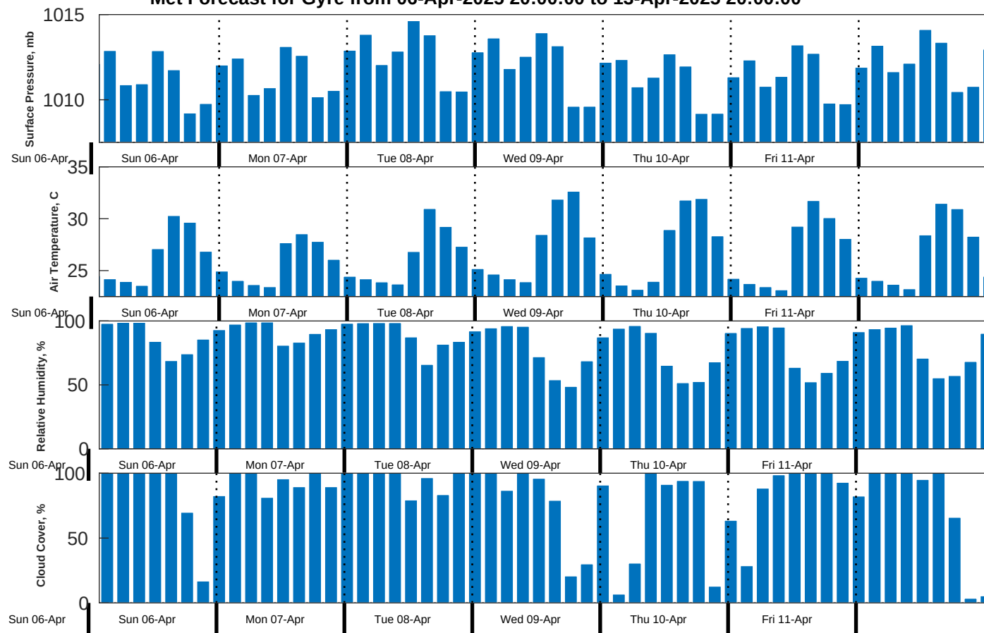
Met Forecast for Gyre from 06-Apr-2025 20:00:00 to 13-Apr-2025 20:00:00
