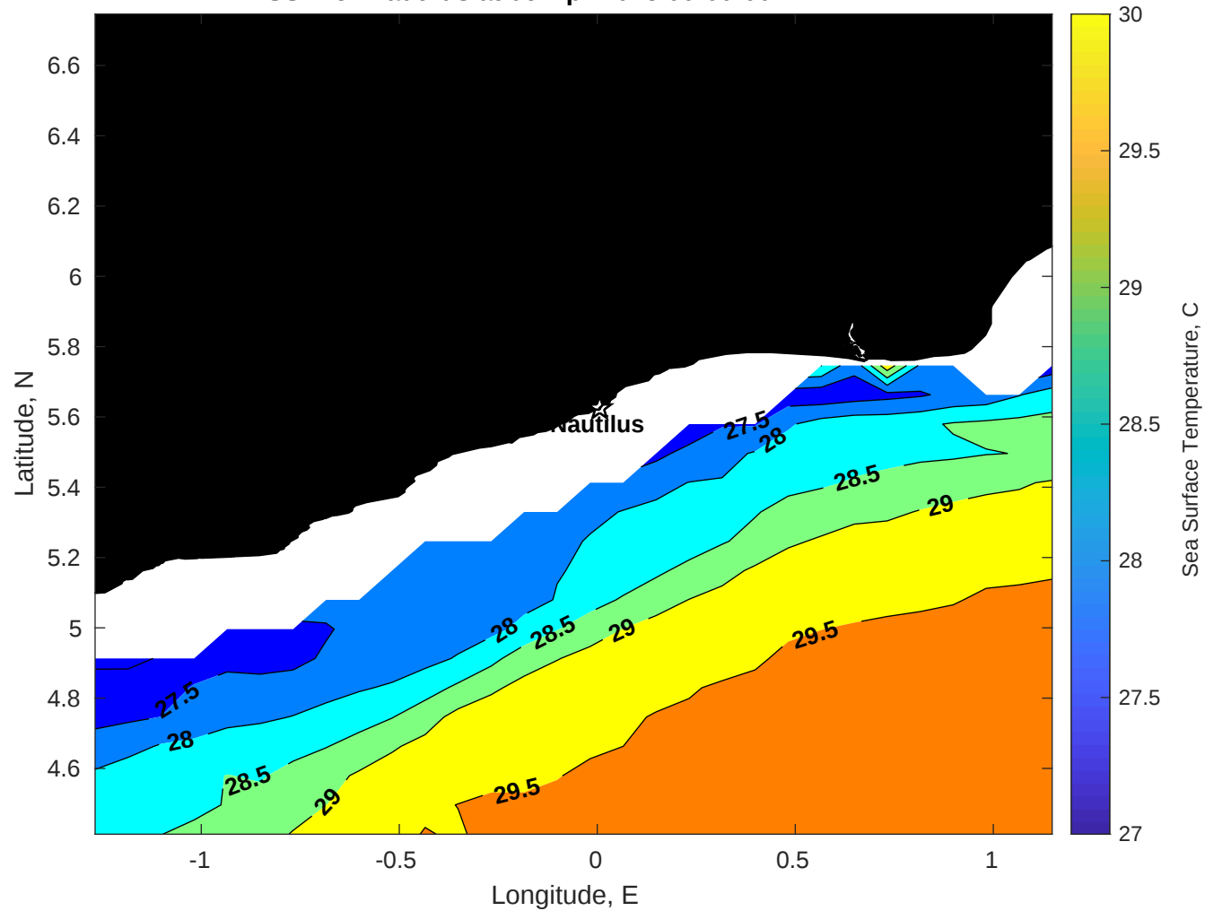
SST for Nautilus at 06-Apr-2025 00:00:00
