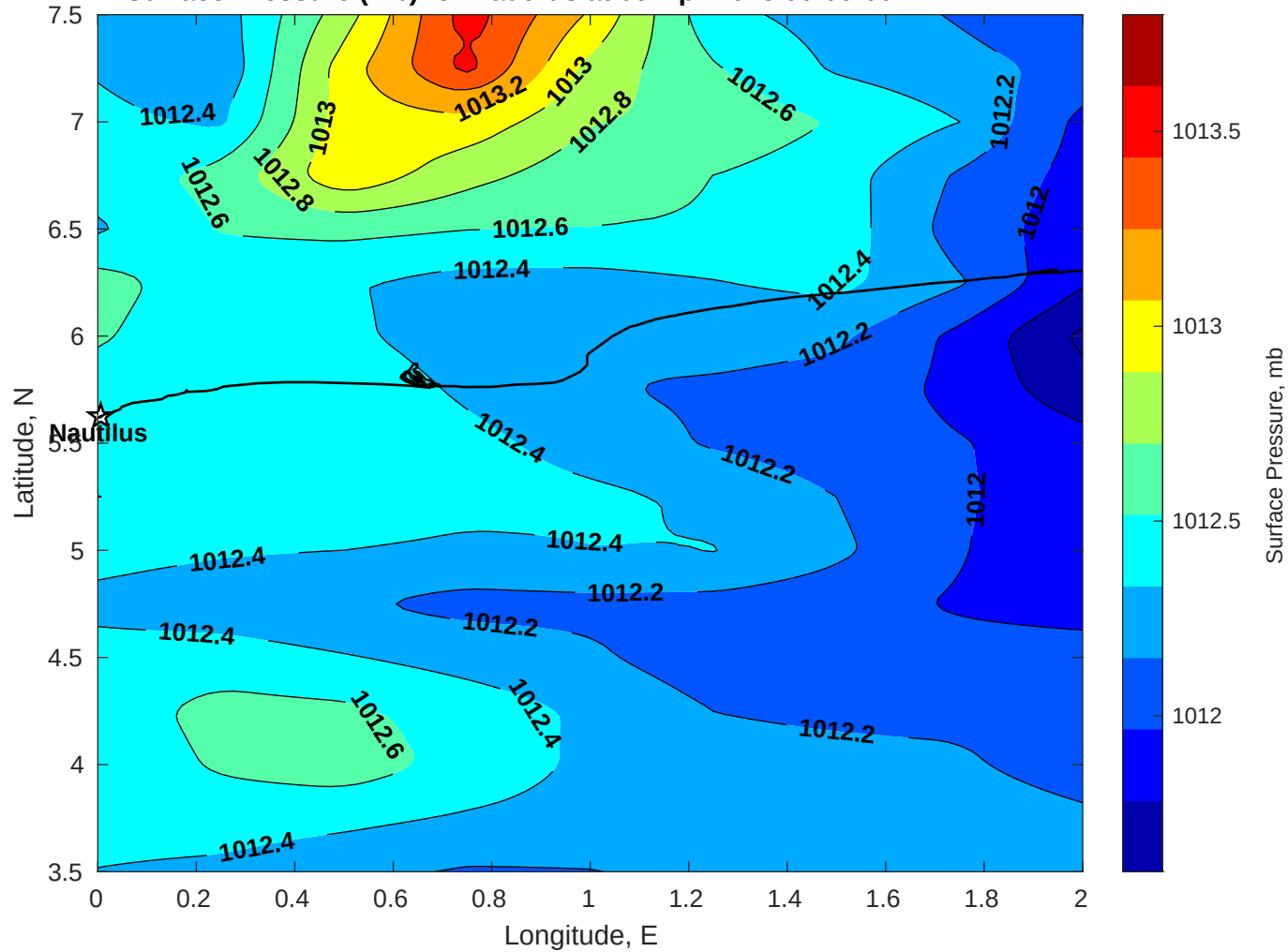
Surface Pressure (mb) for Nautilus at 09-Apr-2025 00:00:00
