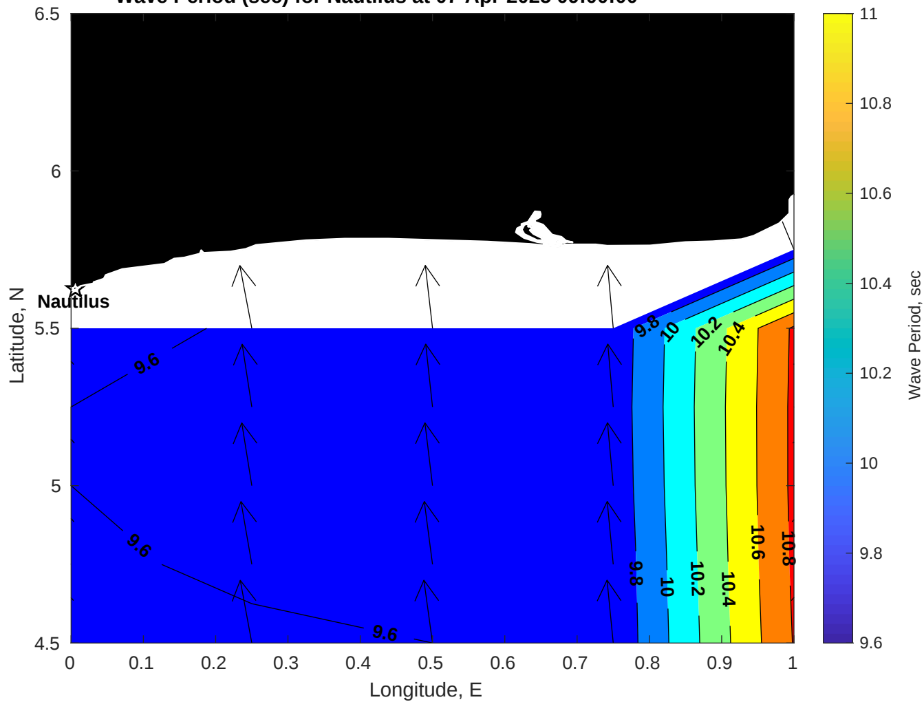
Wave Period (sec) for Nautilus at 07-Apr-2025 09:00:00
