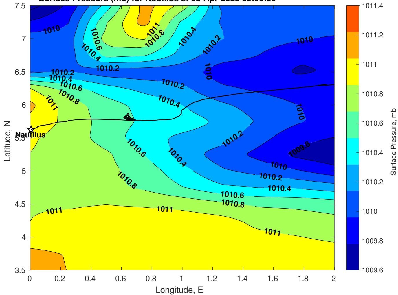
Surface Pressure (mb) for Nautilus at 08-Apr-2025 00:00:00
