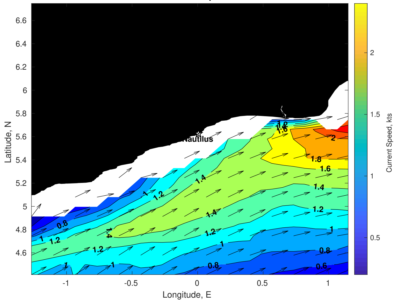
Surface Currents for Nautilus at 06-Apr-2025 00:00:00
