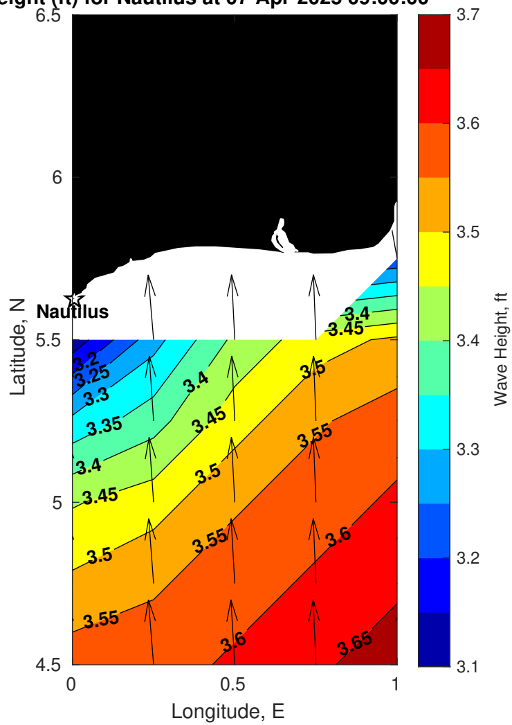
Wave Height (ft) for Nautilus at 07-Apr-2025 09:00:00
