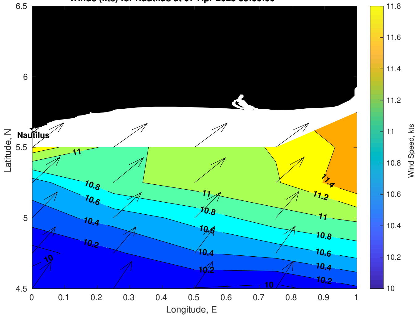
Winds (kts) for Nautilus at 07-Apr-2025 09:00:00
