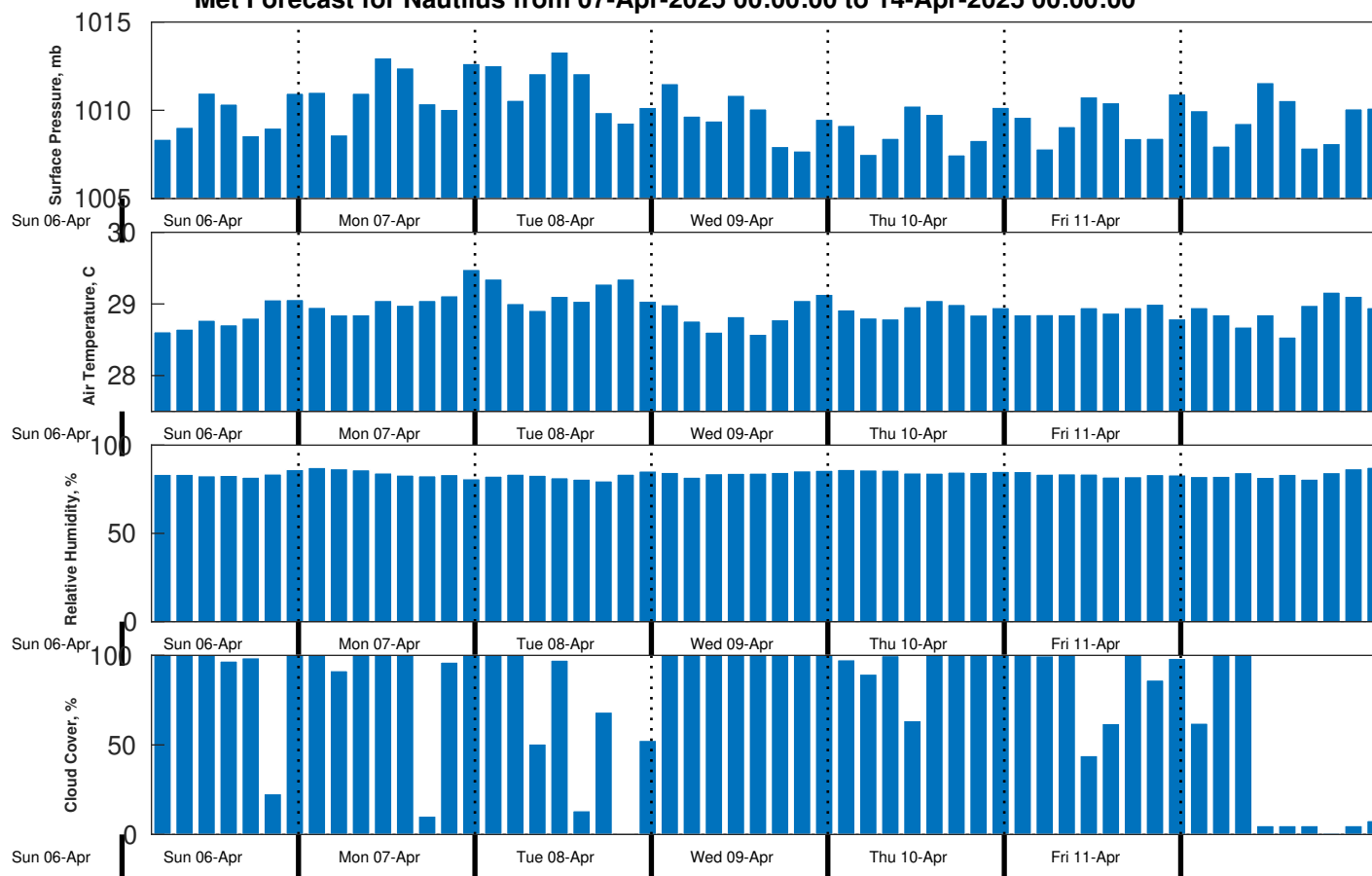
Met Forecast for Nautilus from 07-Apr-2025 00:00:00 to 14-Apr-2025 00:00:00
