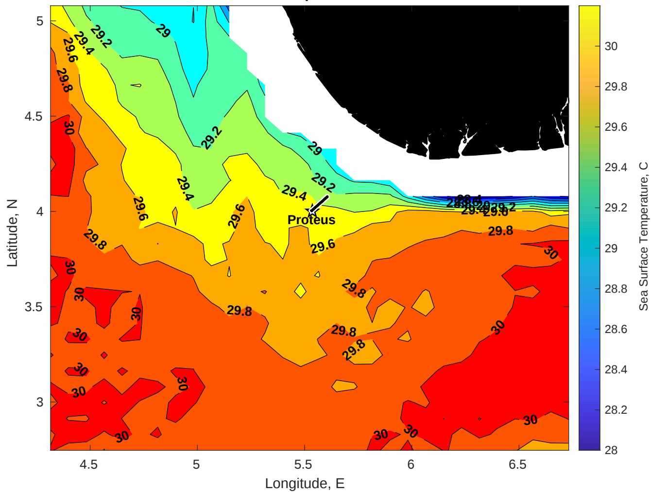
SST for Proteus at 06-Apr-2025 00:00:00
